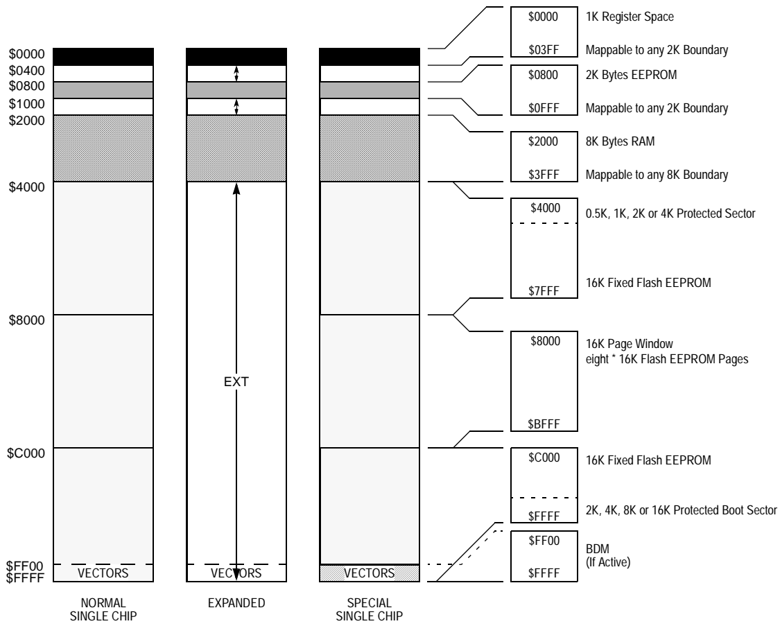
Figure 5 MC9S12Dx128 User Configurable Memory Map
