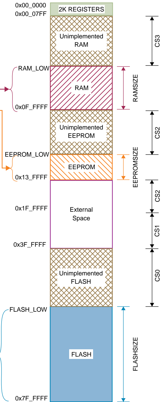
Figure 1-3. S12X CPU & BDM Global Address Mapping
