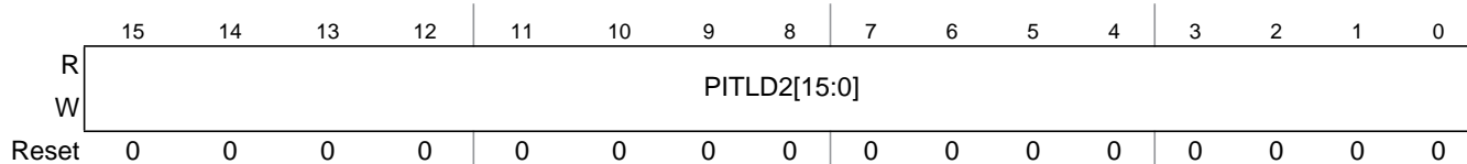
Figure 22-13. PIT Load Register 2 (PITLD2)
