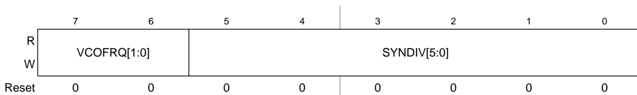
Figure 12-3. CGMIPLL Synthesizer Register (CGMSYNR)
