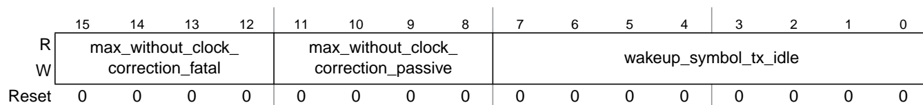
Figure 13-73. Protocol Configuration Register 8 (PCR8)
