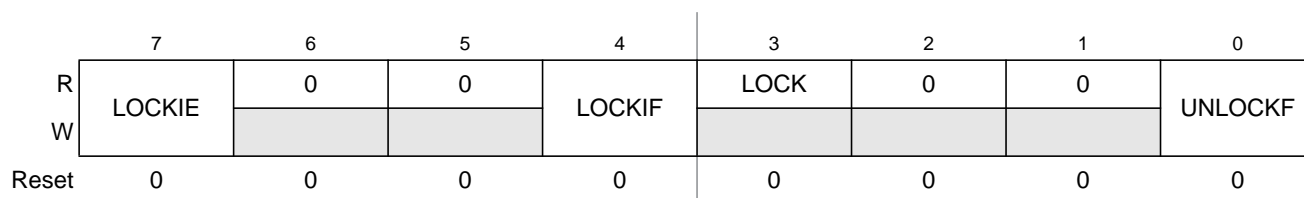
Figure 12-5. CGMIPLL Flags Register (CGMFLG)
