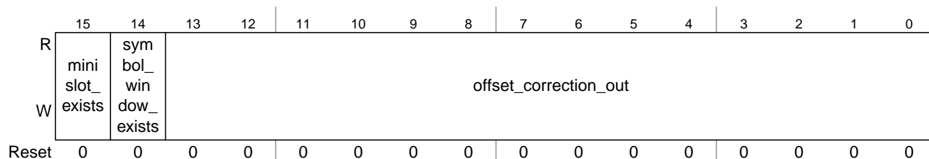
Figure 13-74. Protocol Configuration Register 9 (PCR9)
