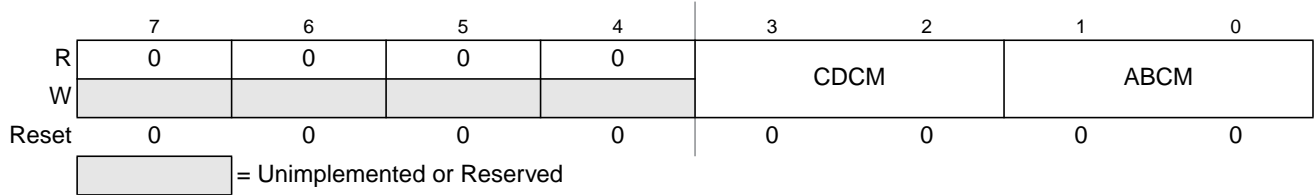
Figure 16-6. Debug Control Register2 (DBGCR2)
