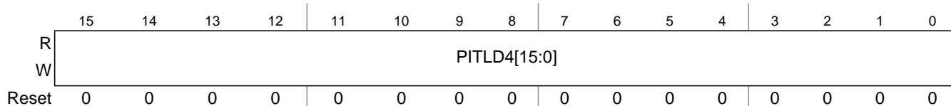
Figure 22-15. PIT Load Register 4 (PITLD4)
