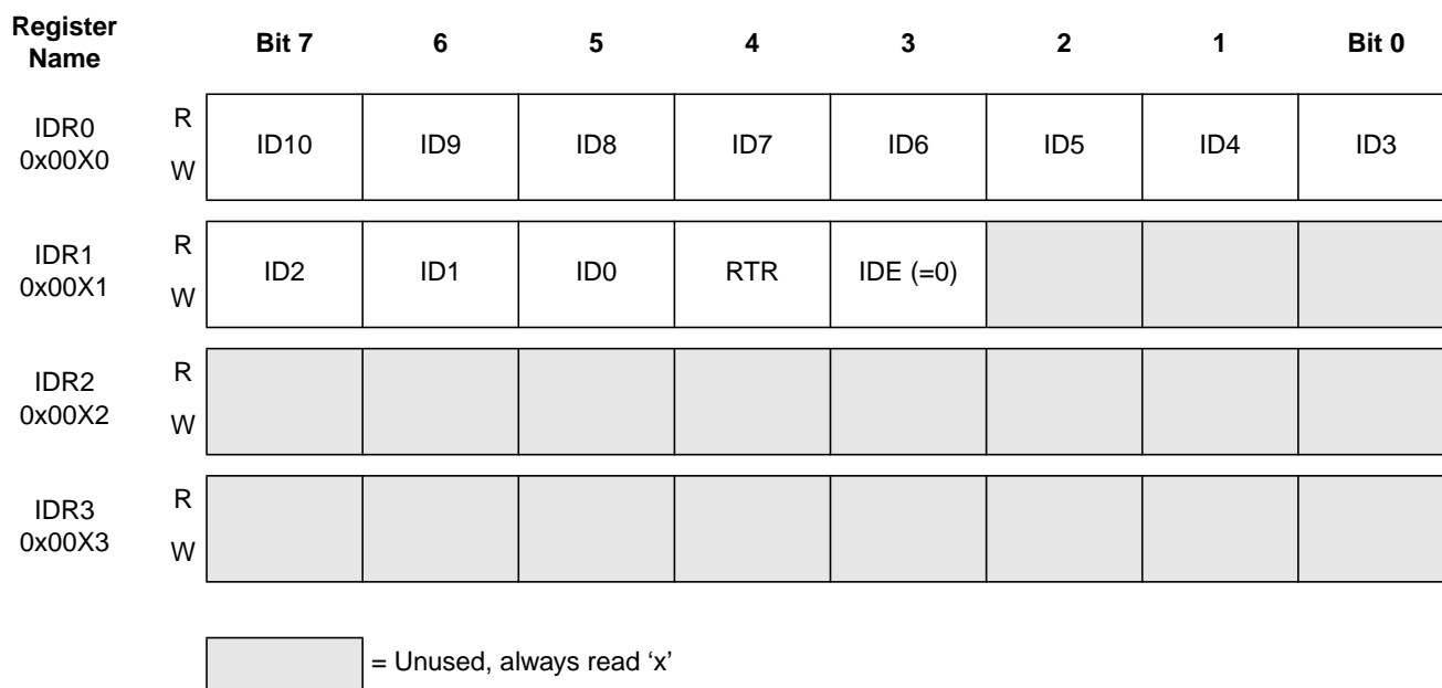
Figure 21-24. Receive/Transmit Message Buffer — Standard Identifier Mapping
