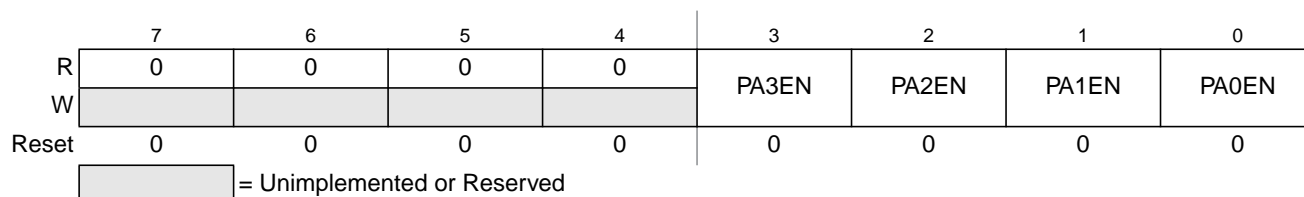
Figure 26-44. Input Control Pulse Accumulators Register (ICPAR)
