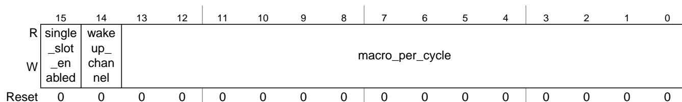
Figure 13-75. Protocol Configuration Register 10 (PCR10)
