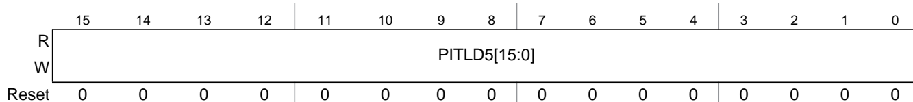
Figure 22-16. PIT Load Register 5 (PITLD5)
