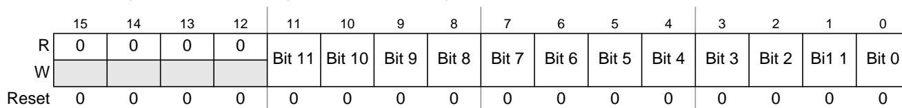
Figure 24-15. Right justified ATD conversion result register (ATDDR n )
