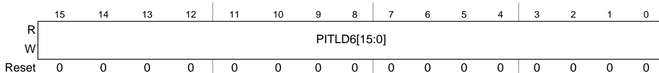
Figure 22-17. PIT Load Register 6 (PITLD6)
