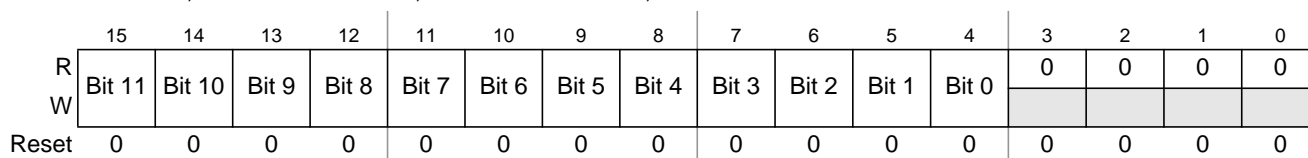
Figure 24-14. Left justified ATD conversion result register (ATDDR n )
