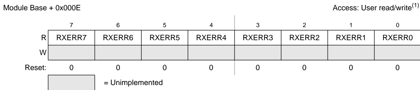
Figure 21-17. MSCAN Receive Error Counter (CANRXERR)
