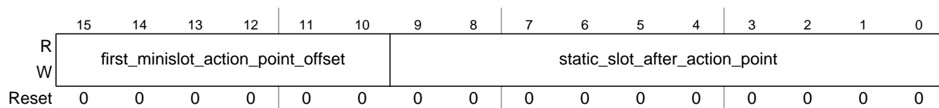
Figure 13-78. Protocol Configuration Register 13 (PCR13)
