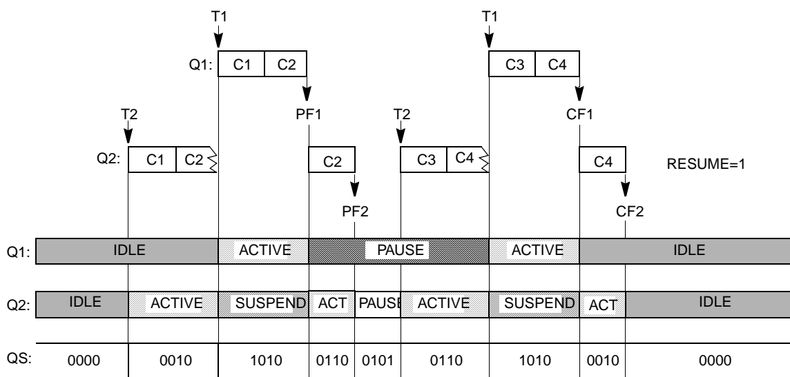
Figure 28-31. CCW Priority Situation 9
