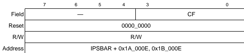
Figure 20-14. GPT Flag Register 1 (GPTFLG1)
