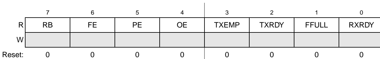
Figure 23-5. UART Status Registers (USR n )
