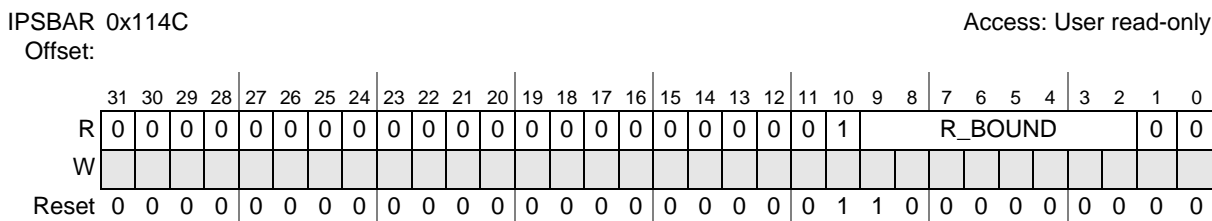
Figure 17-20. FIFO Receive Bound Register (FRBR)
