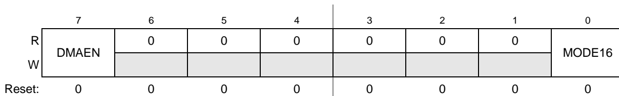
Figure 21-3. DTXMR n Registers
