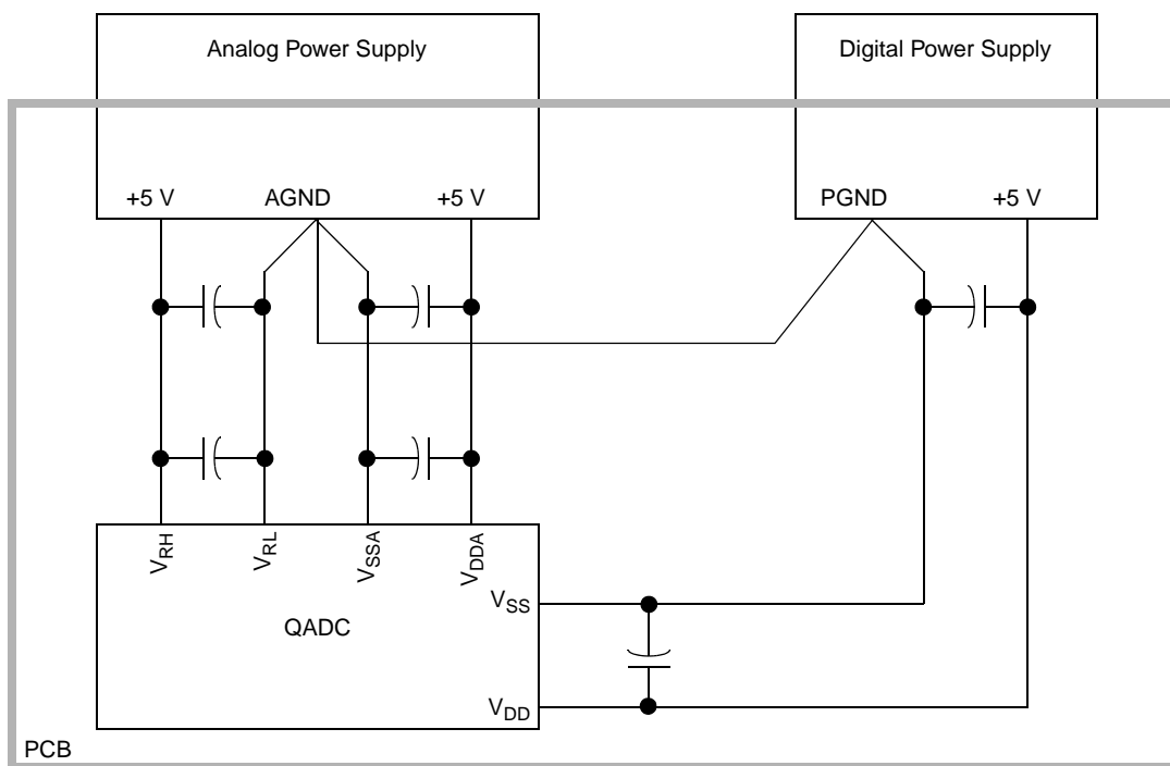
Figure 28-49. Star-Ground at the Point of Power Supply Origin
