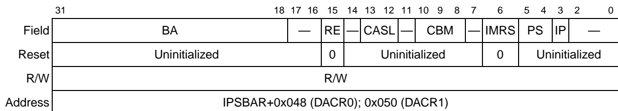
Figure 15-3. DRAM Address and Control Register (DACR n )
