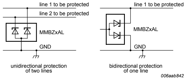
Fig. 15. Application diagram
