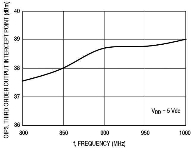
Figure 19. Third Order Output Intercept Point versus Frequency
