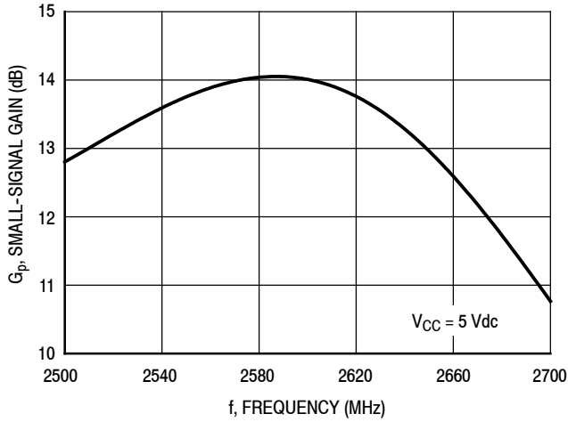
Figure 30. Small-Signal Gain (S21) versus Frequency
