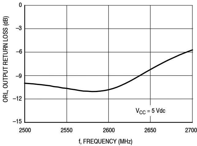
Figure 32. Output Return Loss (S22) versus Frequency
