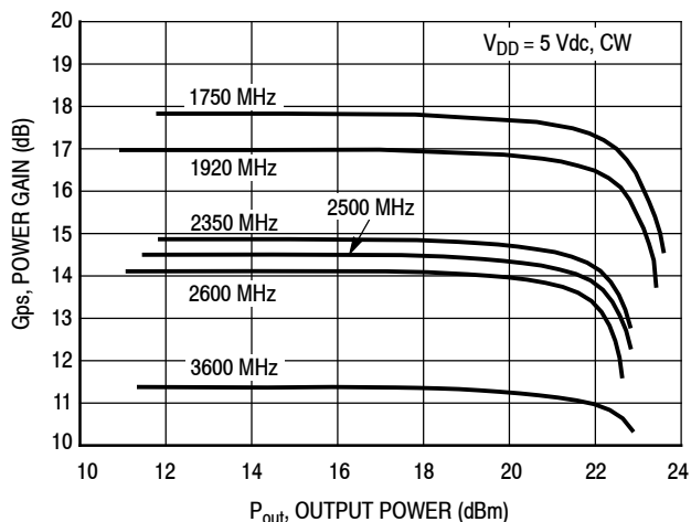
Figure 24. Power Gain versus Output Power and Frequency
