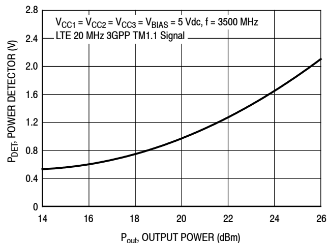
Figure 48. Power Detector versus Output Power
