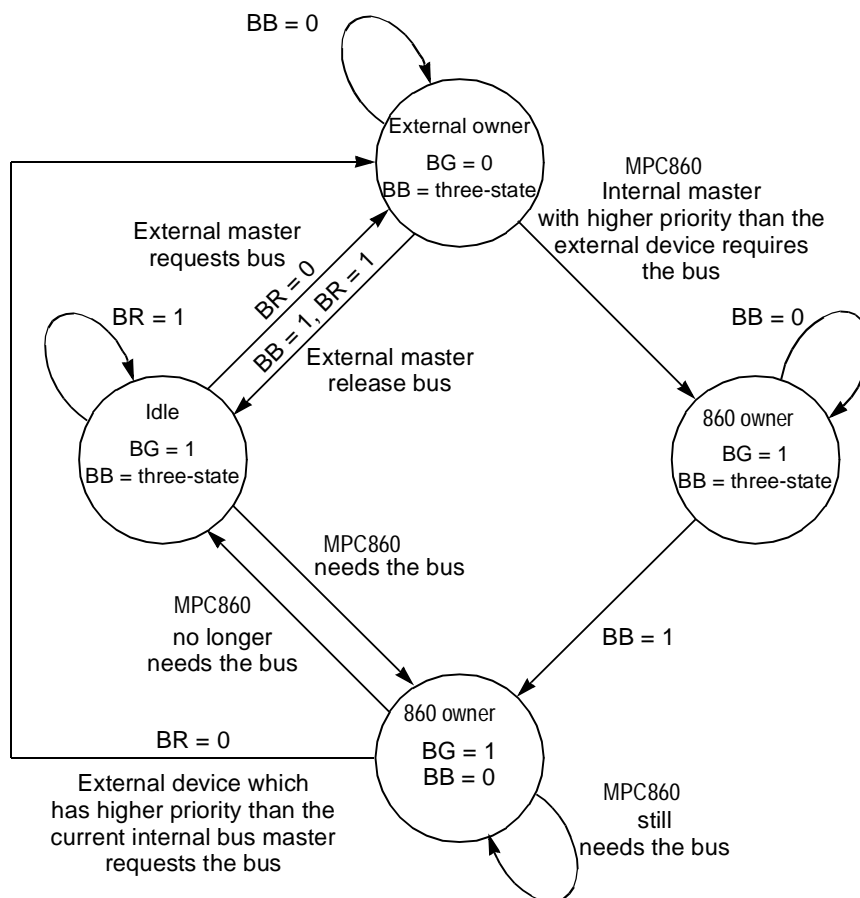
Figure 14-24. Internal Bus Arbitration State Machine
