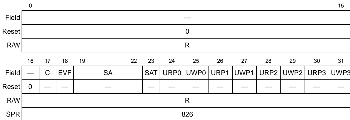
Figure 8-22. DMMU RAM Entry Read Register 1 (MD_RAM1)
