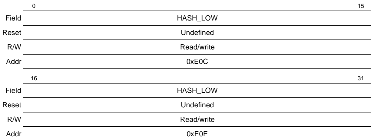
Figure 43-7. HASH_TABLE_LOW Register
