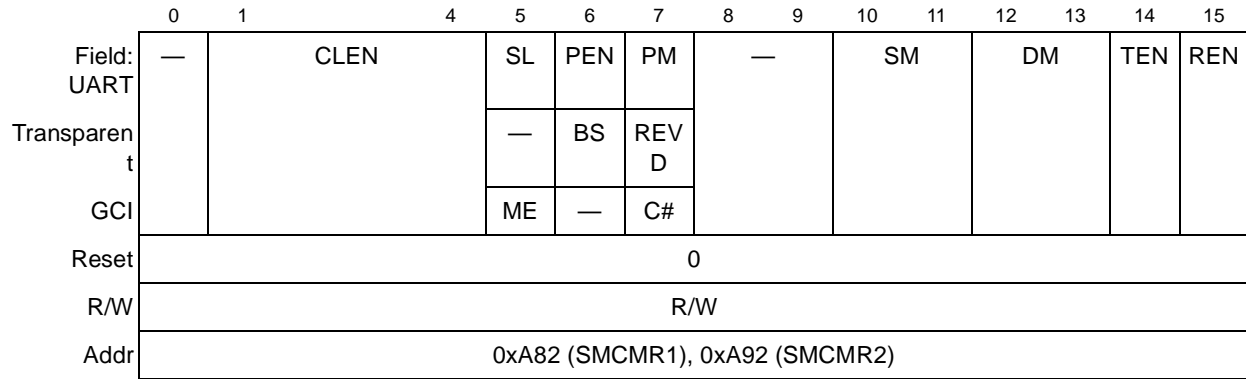
Figure 29-2. SMC Mode Registers (SMCMRn)
