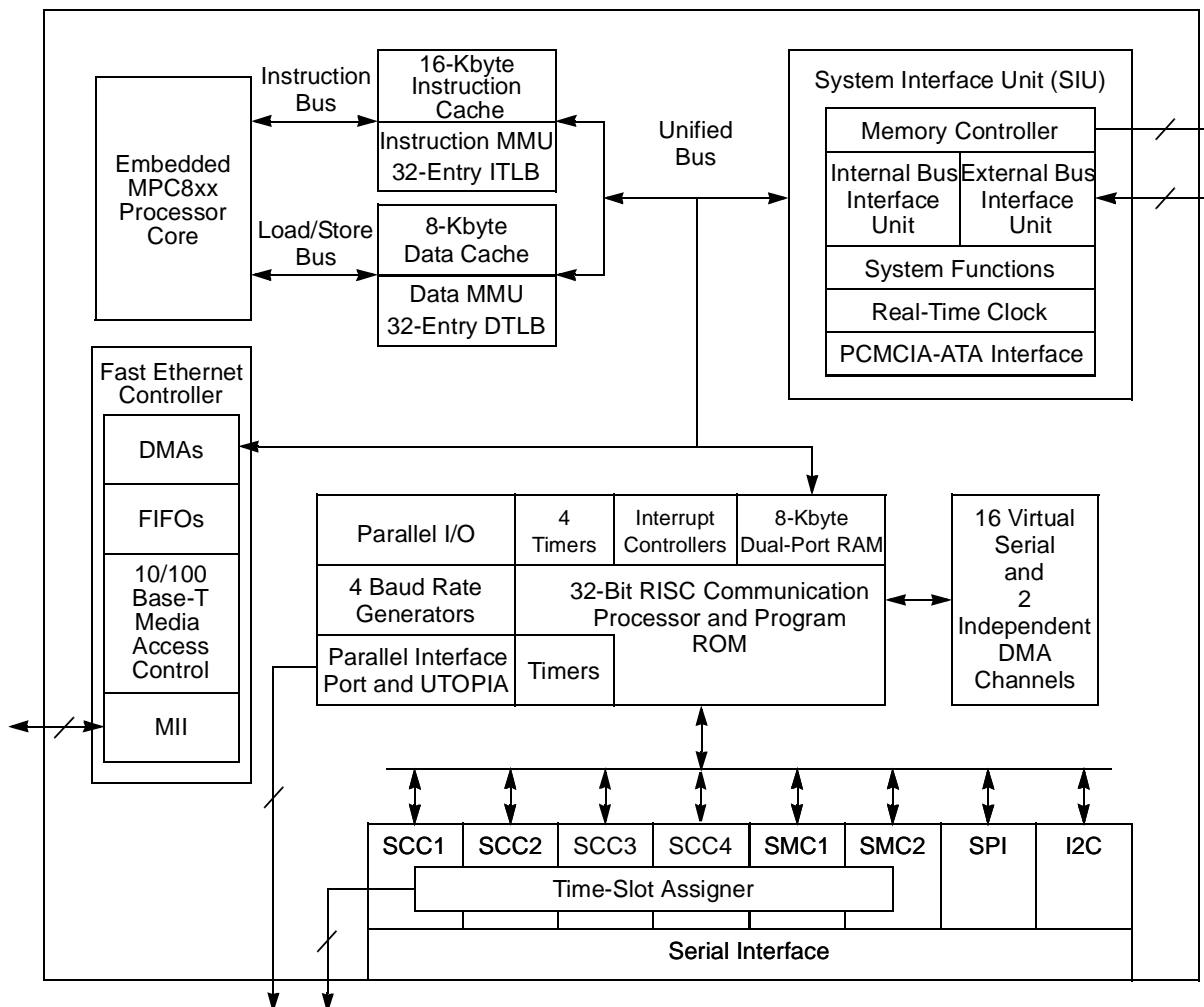
Figure 1-1. MPC860P Block Diagram
