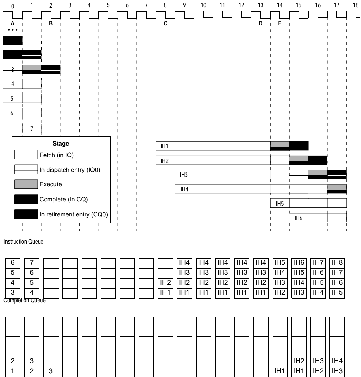
Figure 6-1. Exception Latency
