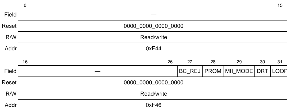
Figure 43-23. R_CNTRL Register
