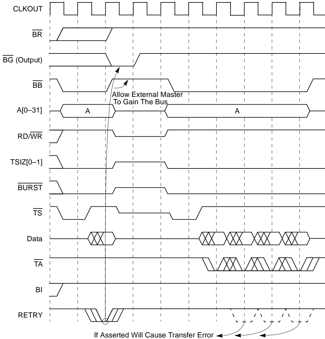
Figure 13-31. \overline{\text{RETRY}} on \overline{\text{BURST}} Cycle
