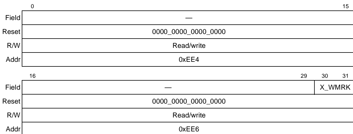
Figure 43-20. X_WMRK Register
