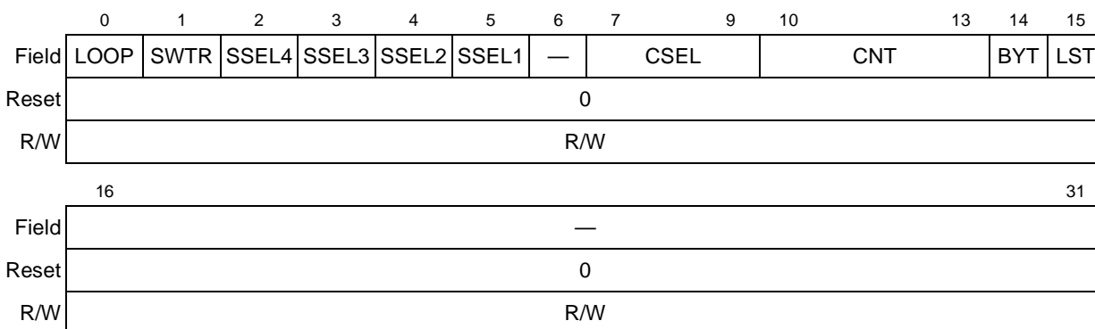
Figure 20-10. SIRAM Entry
