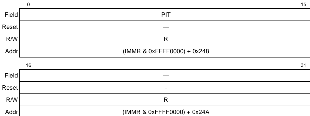
Figure 10-31. PIT Register (PITR)
