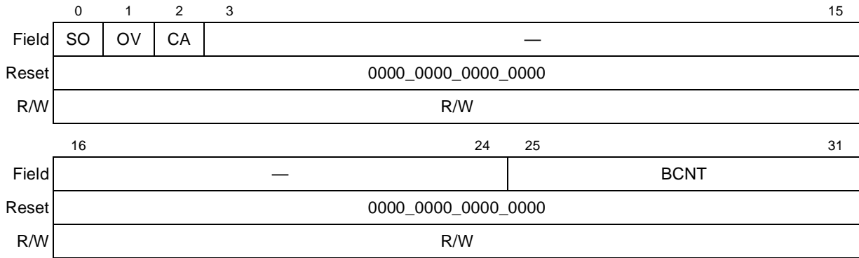
Figure 4-2. XER Register
