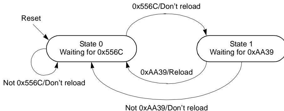
Figure 10-15. Software Watchdog Timer Service State Diagram
