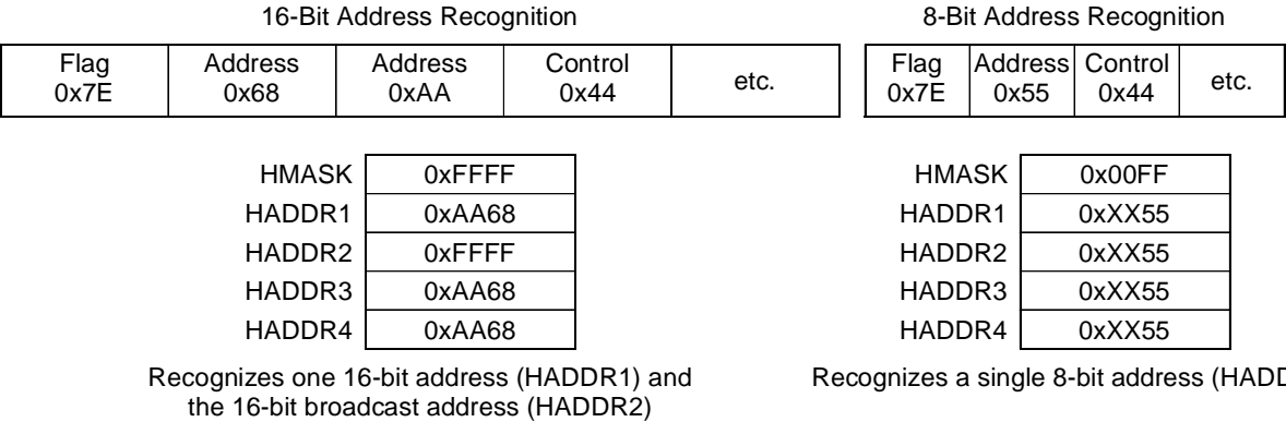
Figure 23-2. HDLC Address Recognition
