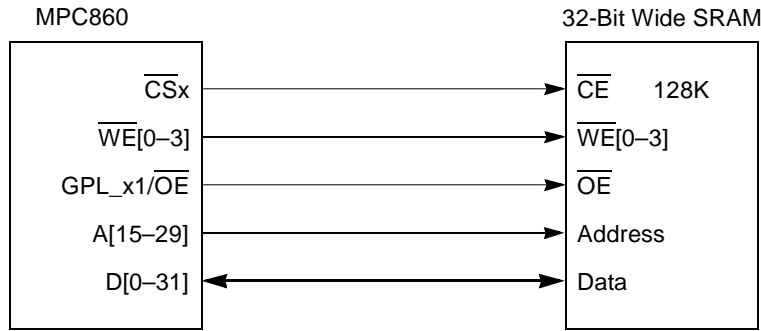
Figure 15-15. GPCM-to-SRAM Configuration
