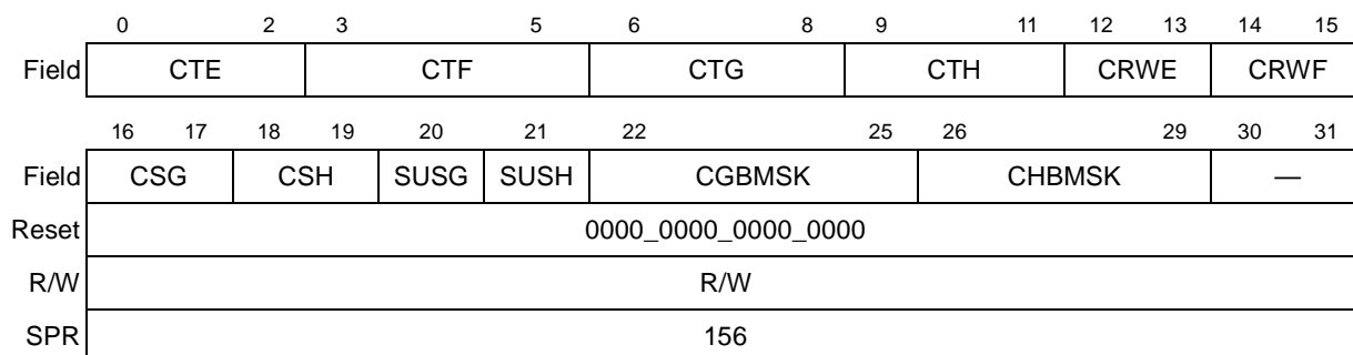
Figure 44-19. Load/Store Support Comparators Control Register (LCTRL1)
