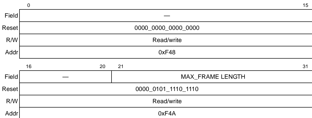
Figure 43-24. R_HASH Register
