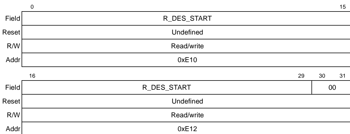
Figure 43-8. R_DES_START Register
