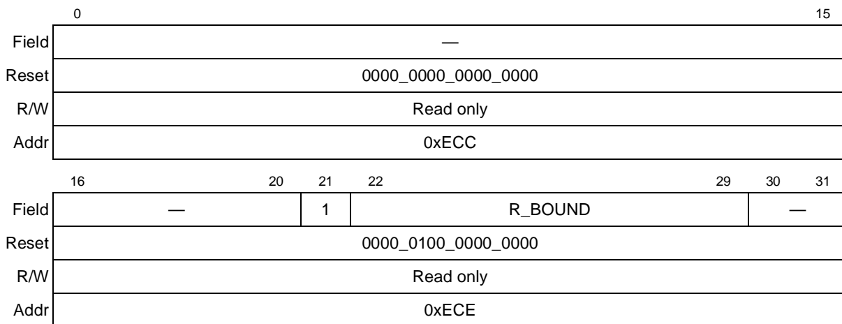
Figure 43-18. R_BOUND Register
