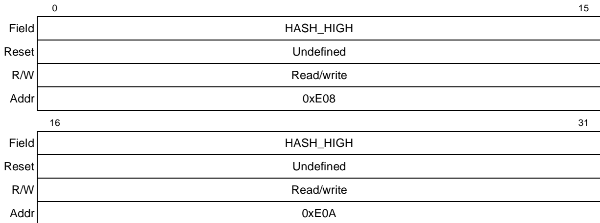
Figure 43-6. HASH_TABLE_HIGH Register
