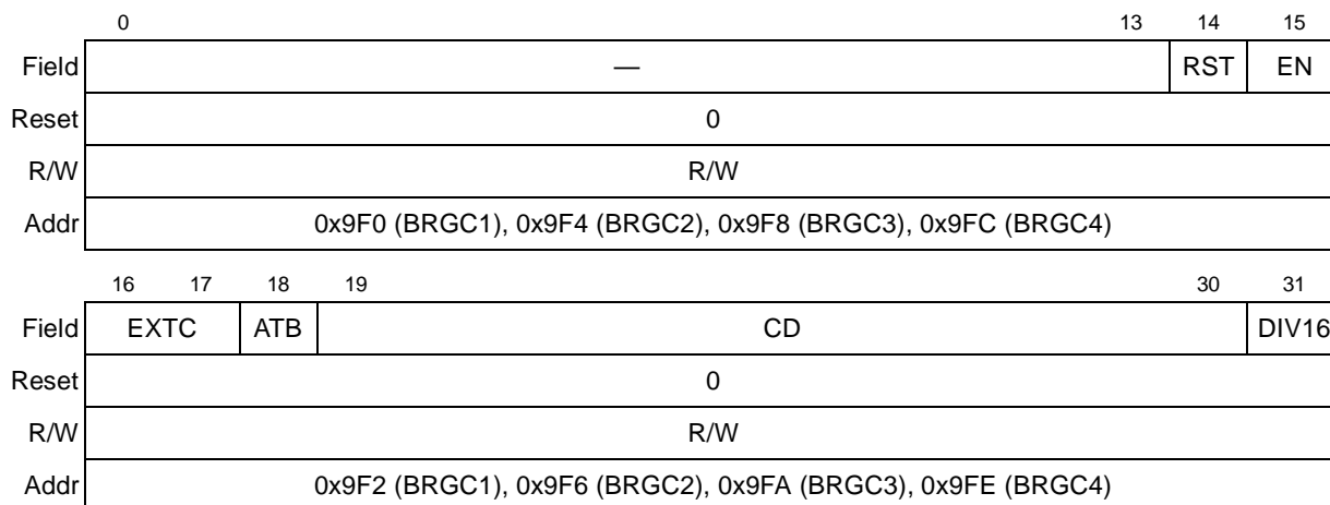
Figure 20-30. Baud Rate Generator Configuration Registers (BRGC n )
