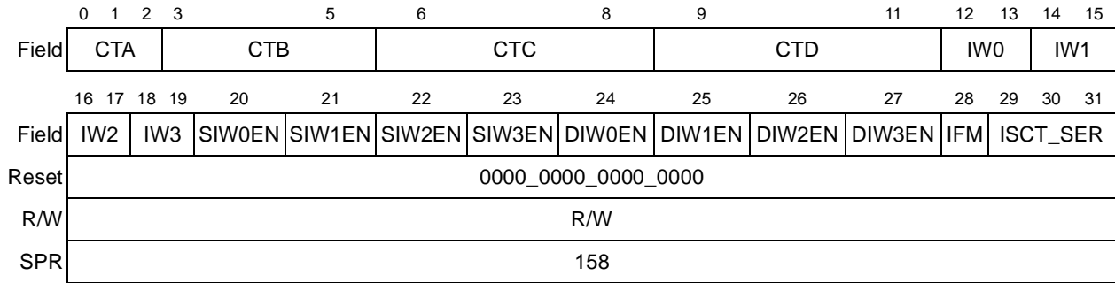
Figure 44-18. Instruction Support Control Register (ICTRL)
