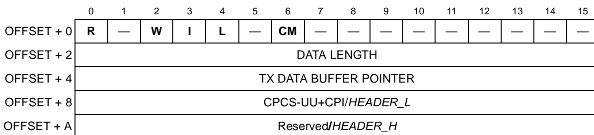
Figure 36-5. ATM TxBD
