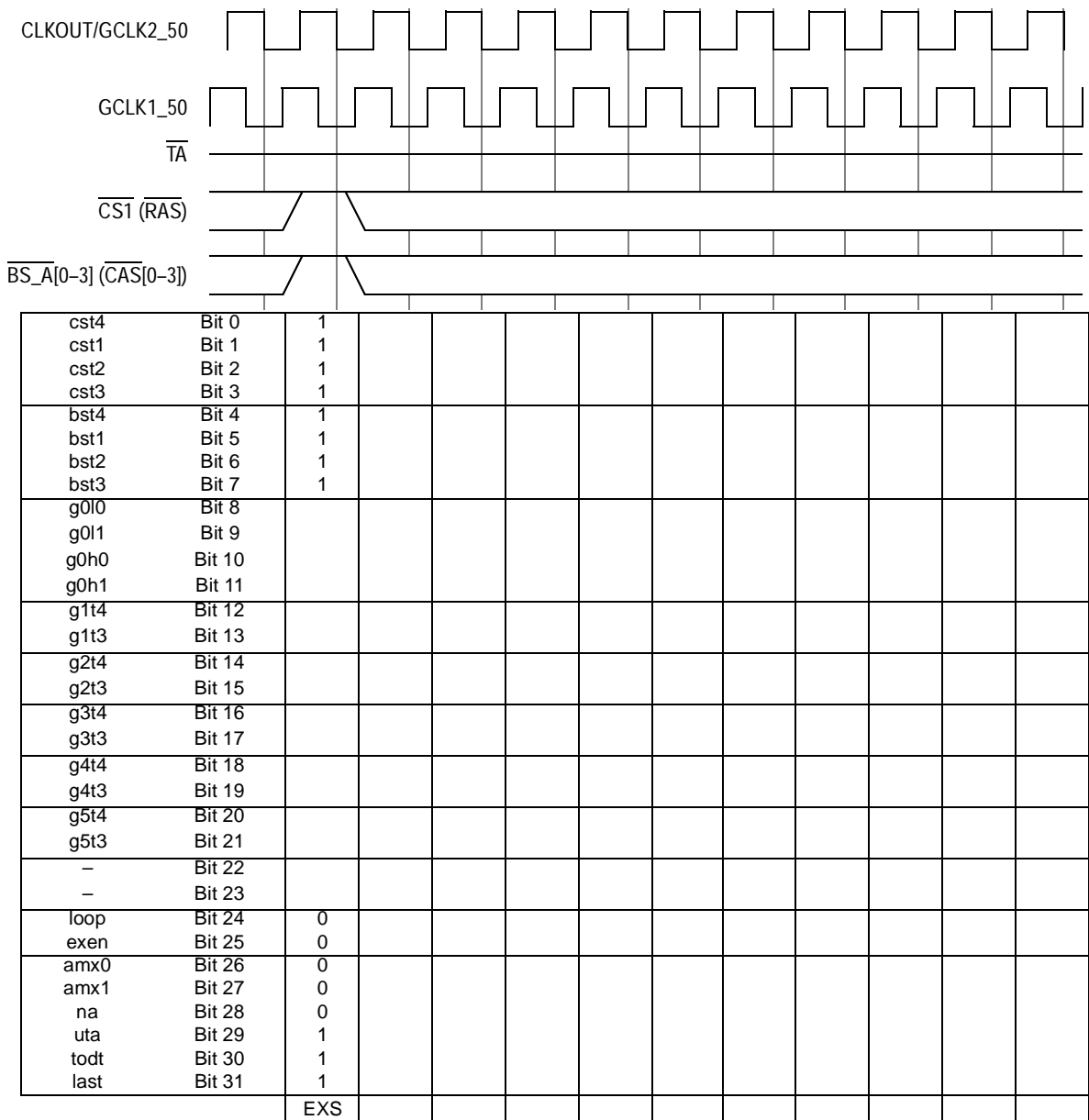
Figure 15-61. Exception Cycle
