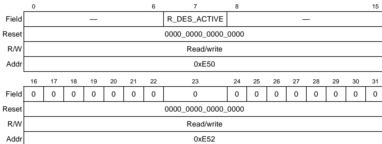
Figure 43-14. R_DES_ACTIVE Register
