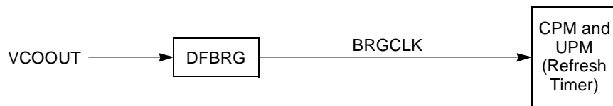
Figure 14-10. BRGCLK Divider
