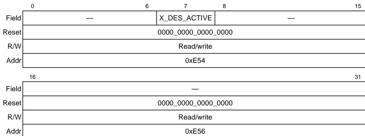
Figure 43-15. X_DES_ACTIVE Register
