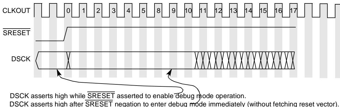
Figure 44-7. Debug Mode Reset Configuration Timing Diagram
