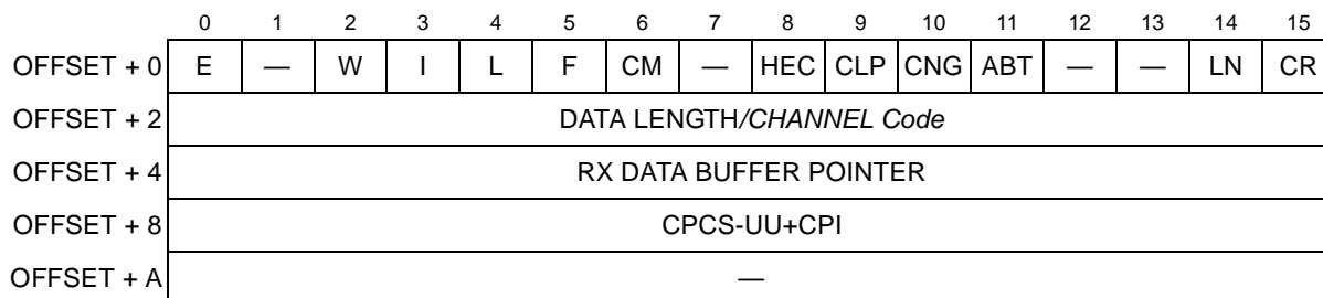
Figure 36-3. ATM RxBd
