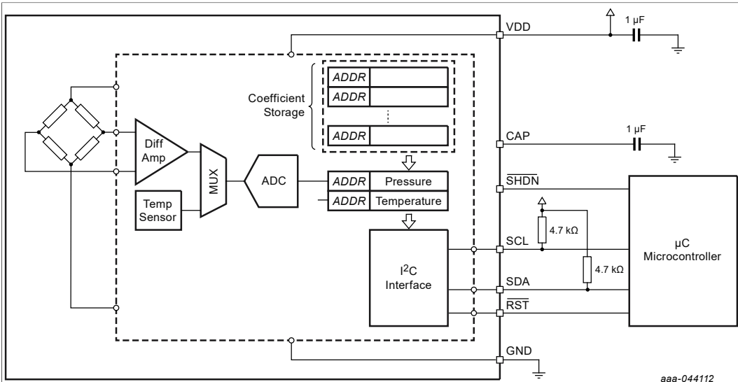
Figure 1. Block diagram of MPL115A2S
