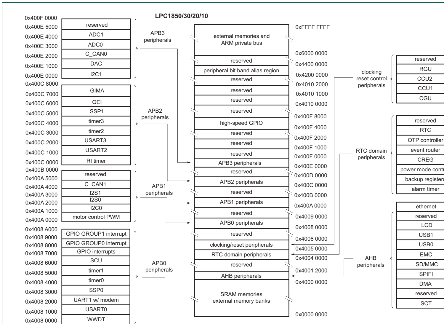
Fig 4. Memory map with peripherals - flashless parts LPC1850/30/20/10 (see Figure 3 for detailed addresses of memory blocks)
