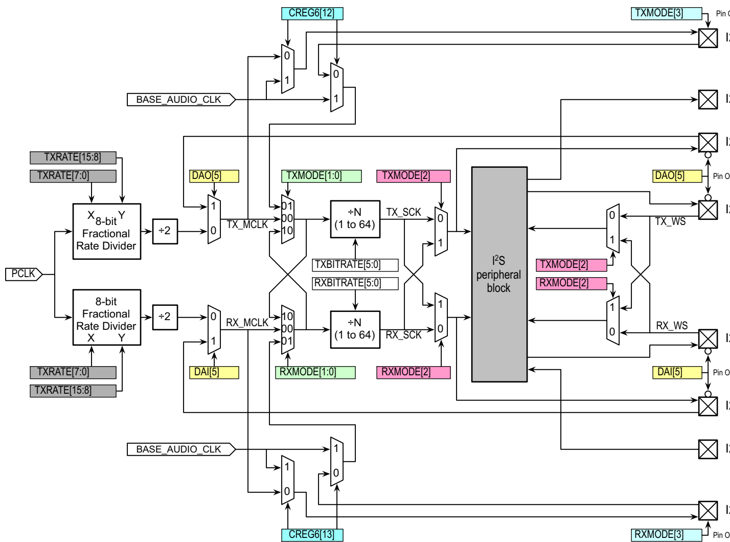
Fig 133. I2S clocking and pin connections
