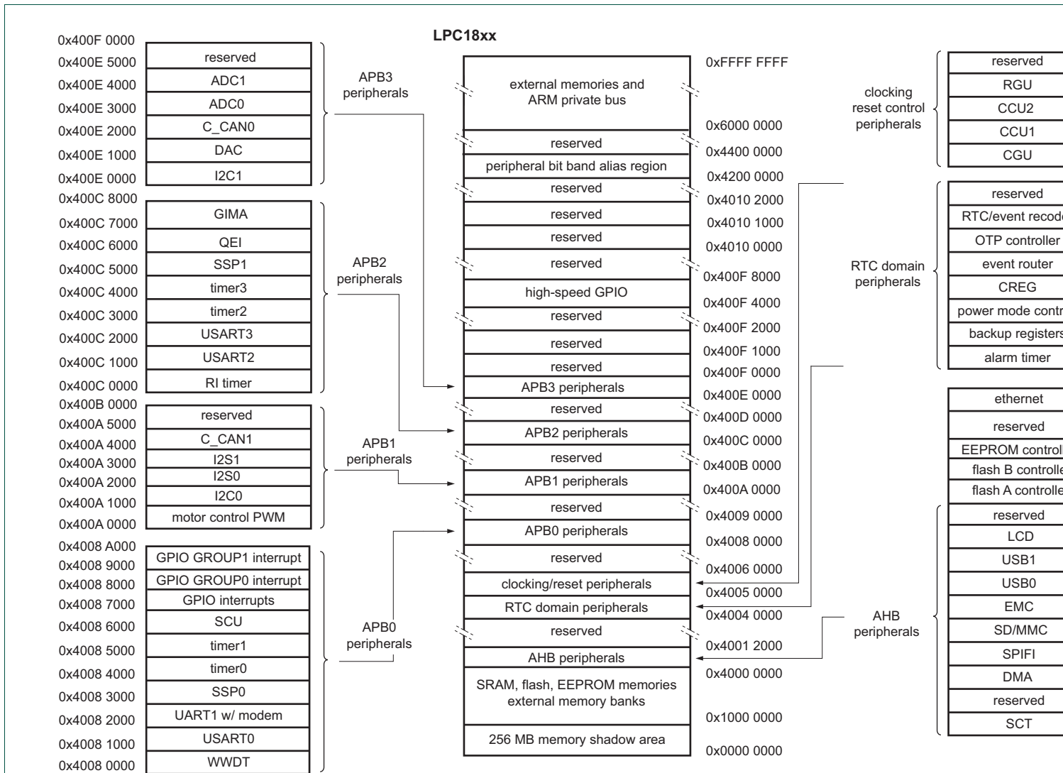
Fig 6. Memory mapping - parts with on-chip flash (peripherals)
