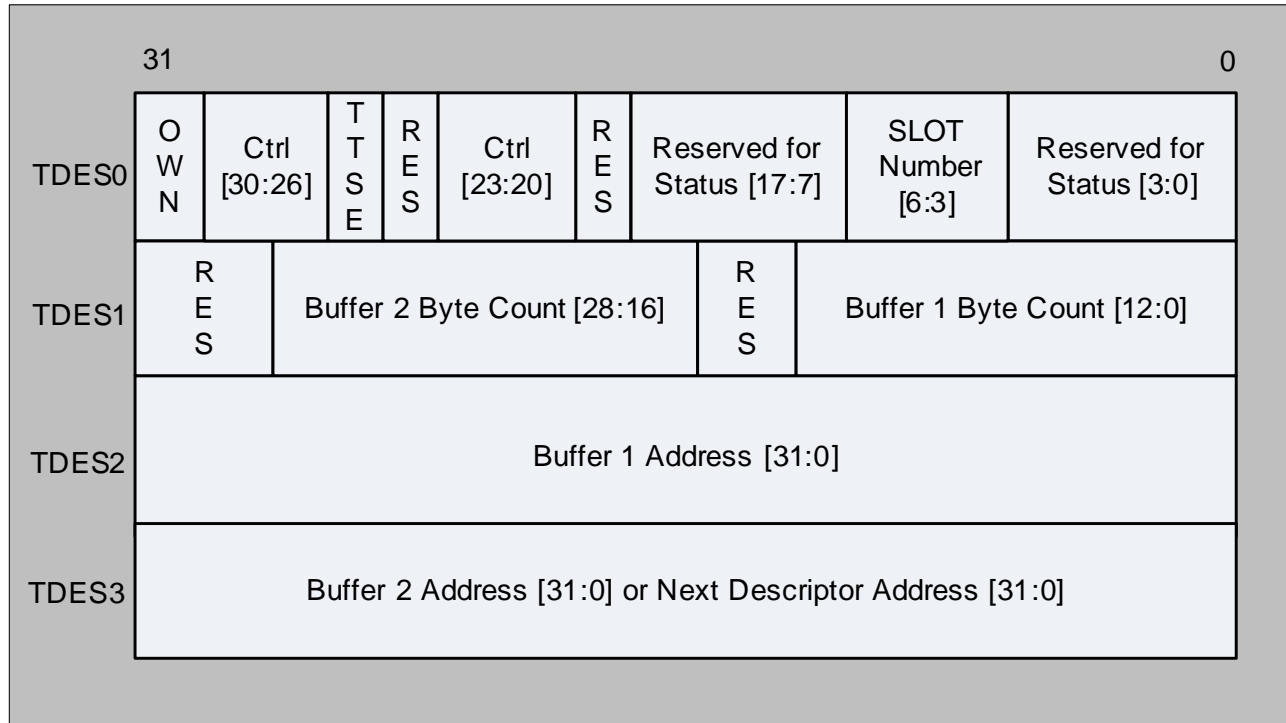
Fig 77. Transmit descriptor fetch (read)
