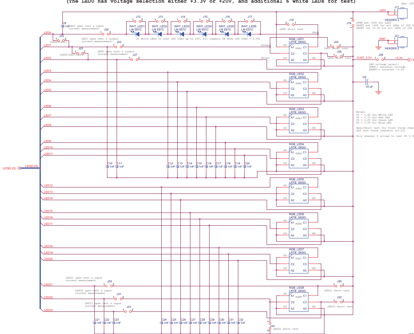
Fig 5. PCA9956B demo board schematic (part B)
