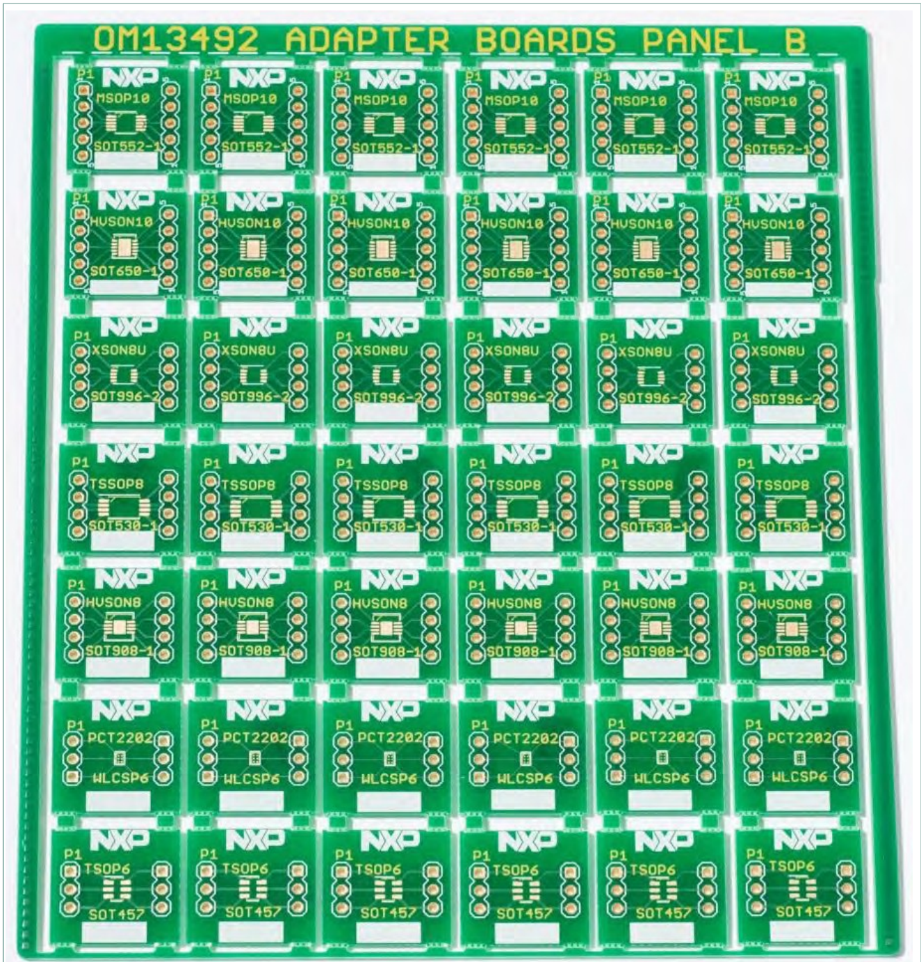
Figure 3. Panel B – consisting of six positions each of MSOP10, HUSON10, XSON8U, TSSOP8, HVSON8, PCT2202 / WLCSP6 and TSOP6
