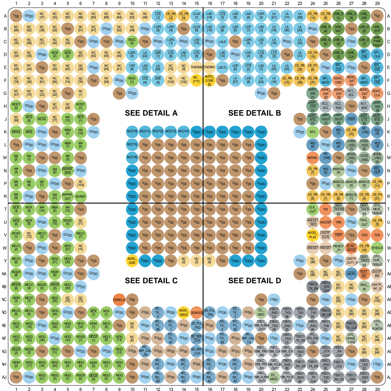
Figure 2. P1012 Top View Ballmap
