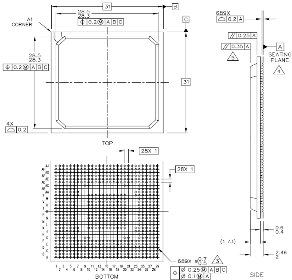
Figure 69. P1012 Package
