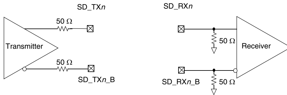
Figure 36. SerDes Transmitter and Receiver Reference Circuits
