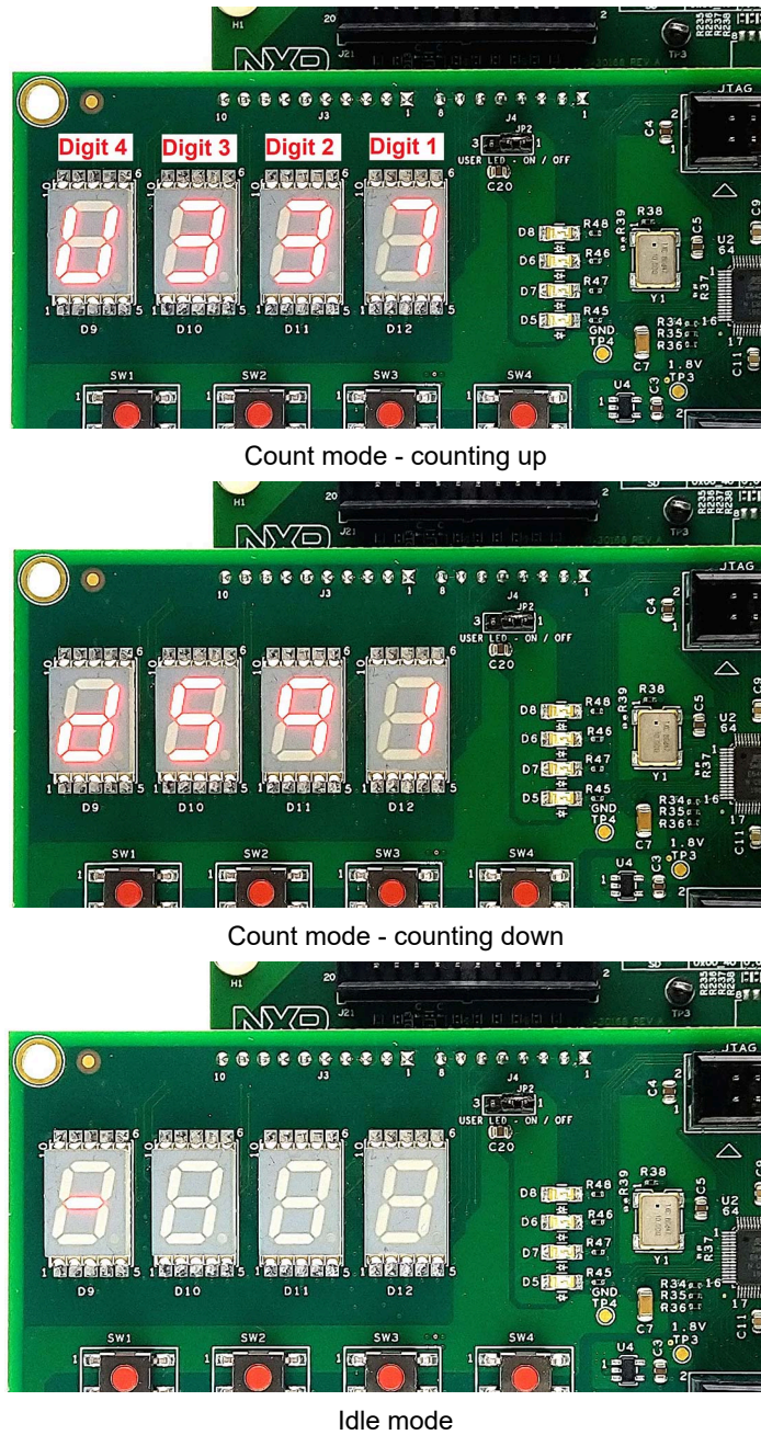
Figure 3. PCAL6524EV-ARD on-board LED display
