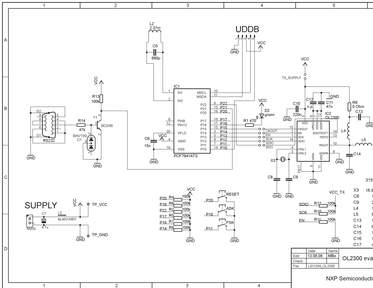
Fig 1. Schematic of OL2300 RF evaluation board
