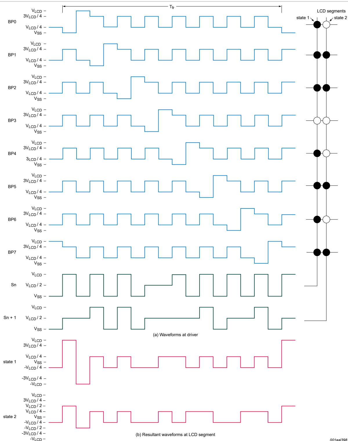
Figure 18. Waveforms for 1:8 multiplex drive mode with bias \frac{1}{4} and line inversion
