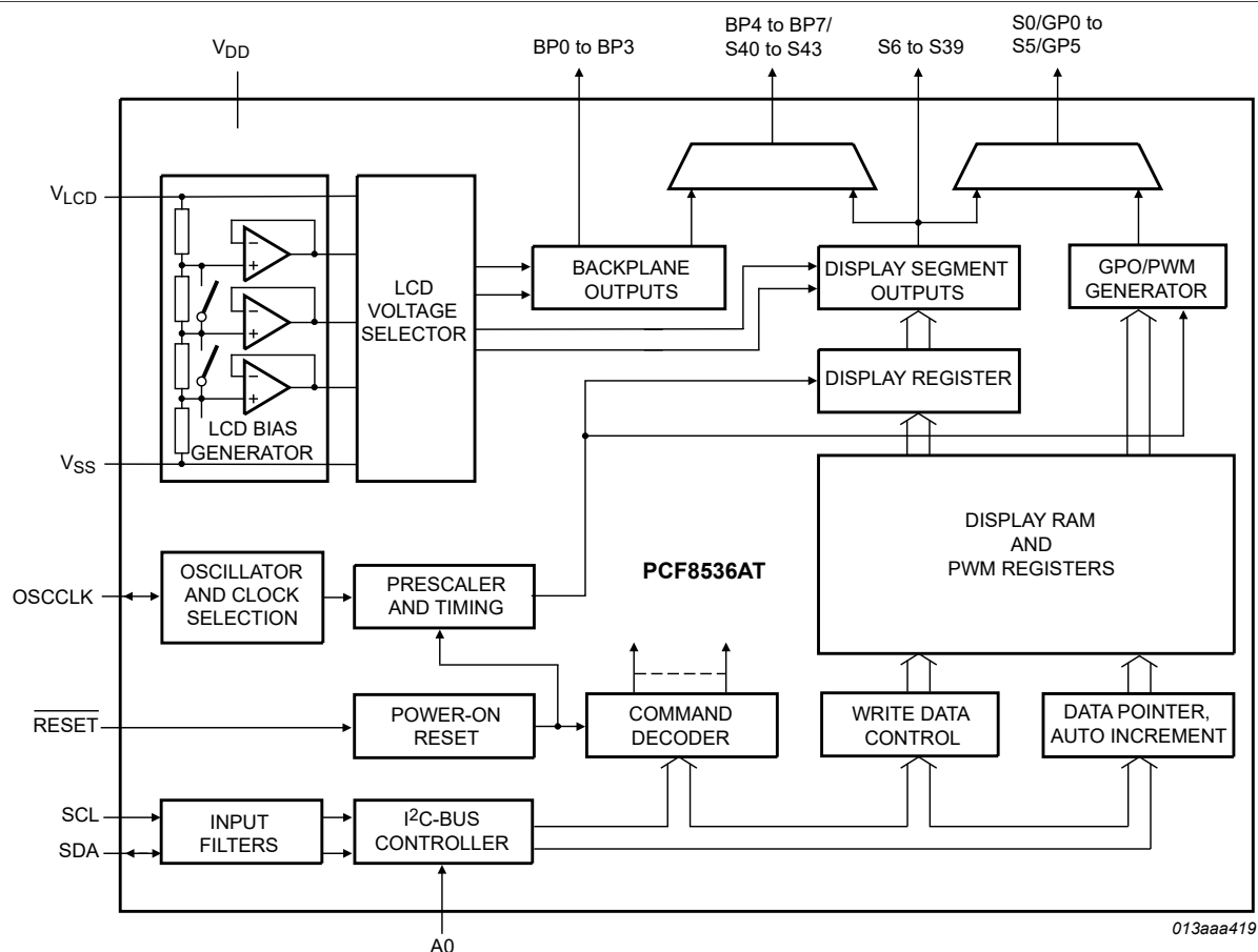
Figure 1. Block diagram of PCF8536AT
