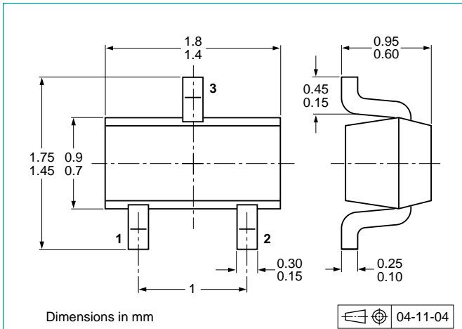
Fig 12. Package outline PDTC144EE (SOT416/SC-75)
