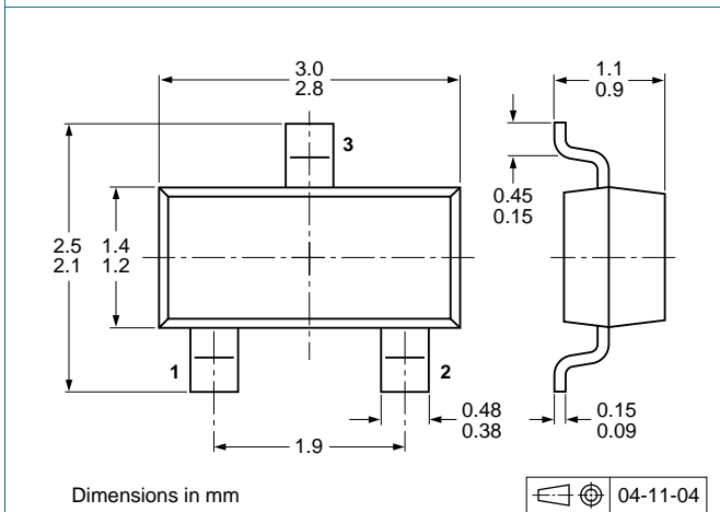
Fig 14. Package outline PDTC144ET (SOT23)
