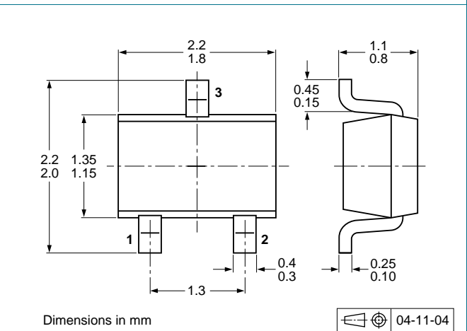
Fig 15. Package outline PDTC144EU (SOT323/SC-70)
