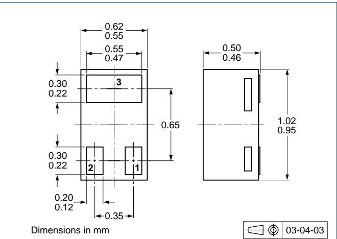
Fig 13. Package outline PDTC144EM (SOT883/SC-101)
