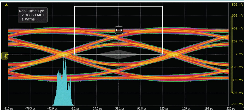
Fig. 9. HDMI 2.0 eye diagram TP1, test board without device; typical values
