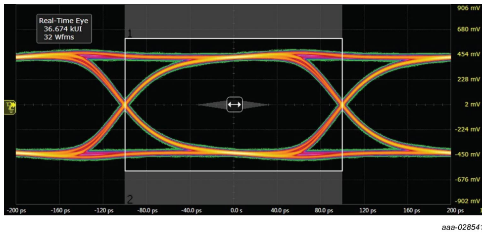
Fig. 7. USB 3.2 eye diagram 5 Gbps, test board without device; typical values
