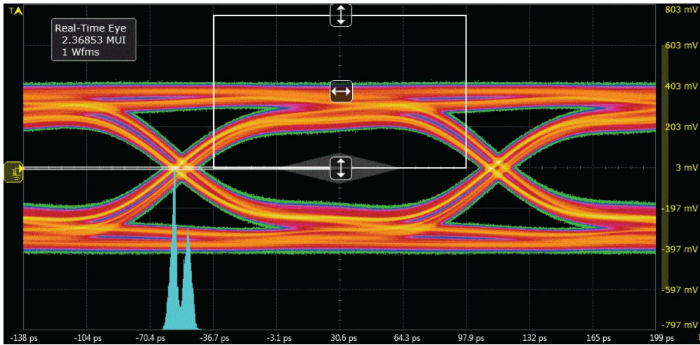
Fig. 8. HDMI 2.0 eye diagram TP1, test board with PCMFxUSB3B/C; typical values
