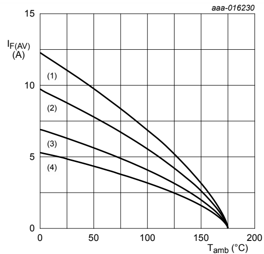
Ceramic PCB, \text{Al}_2\text{O}_3 , standard footprint T_j = 175^\circ\text{C} (1) \delta = 1 ; DC (2) \delta = 0.5 ; f = 20 kHz (3) \delta = 0.2 ; f = 20 kHz (4) \delta = 0.1 ; f = 20 kHz
