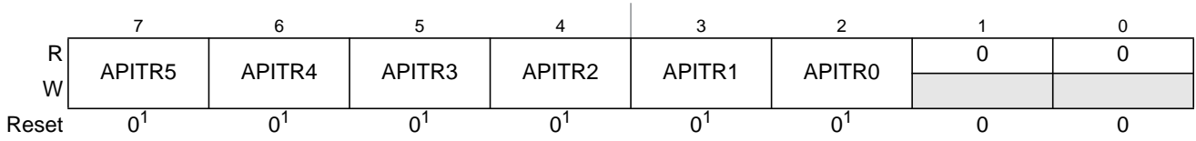
Figure 14-5. Autonomous Periodical Interrupt Trimming Register (VREGAPITR)
