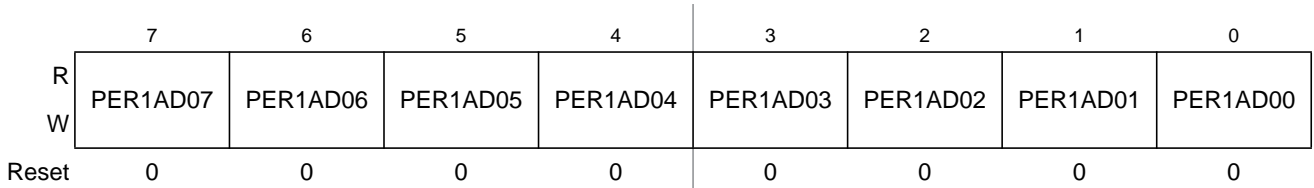
Figure 23-67. Port AD0 Pull Up Enable Register 1 (PER1AD0)
