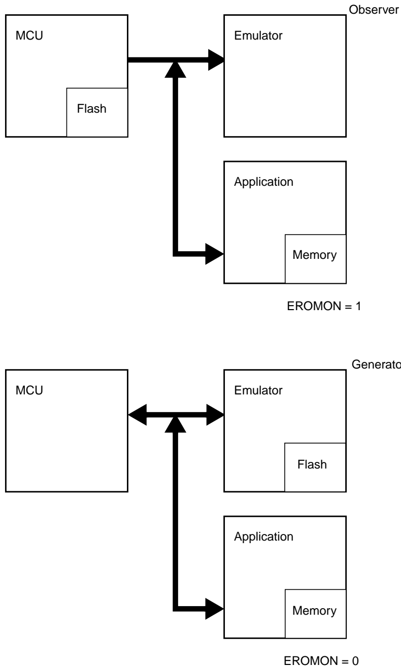
Figure 17-30. ROMON = 1 in Emulation Expanded Mode
