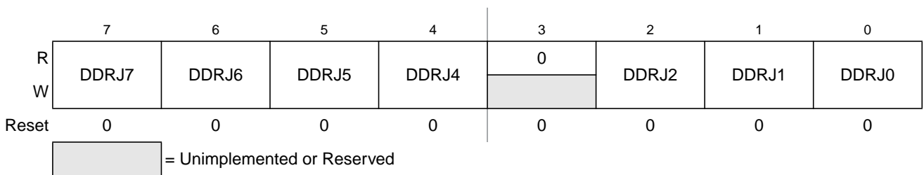
Figure 23-58. Port J Data Direction Register (DDRJ)
