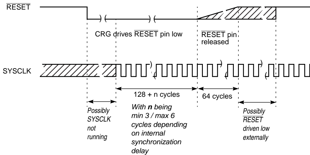
Figure 2-25. RESET Timing
