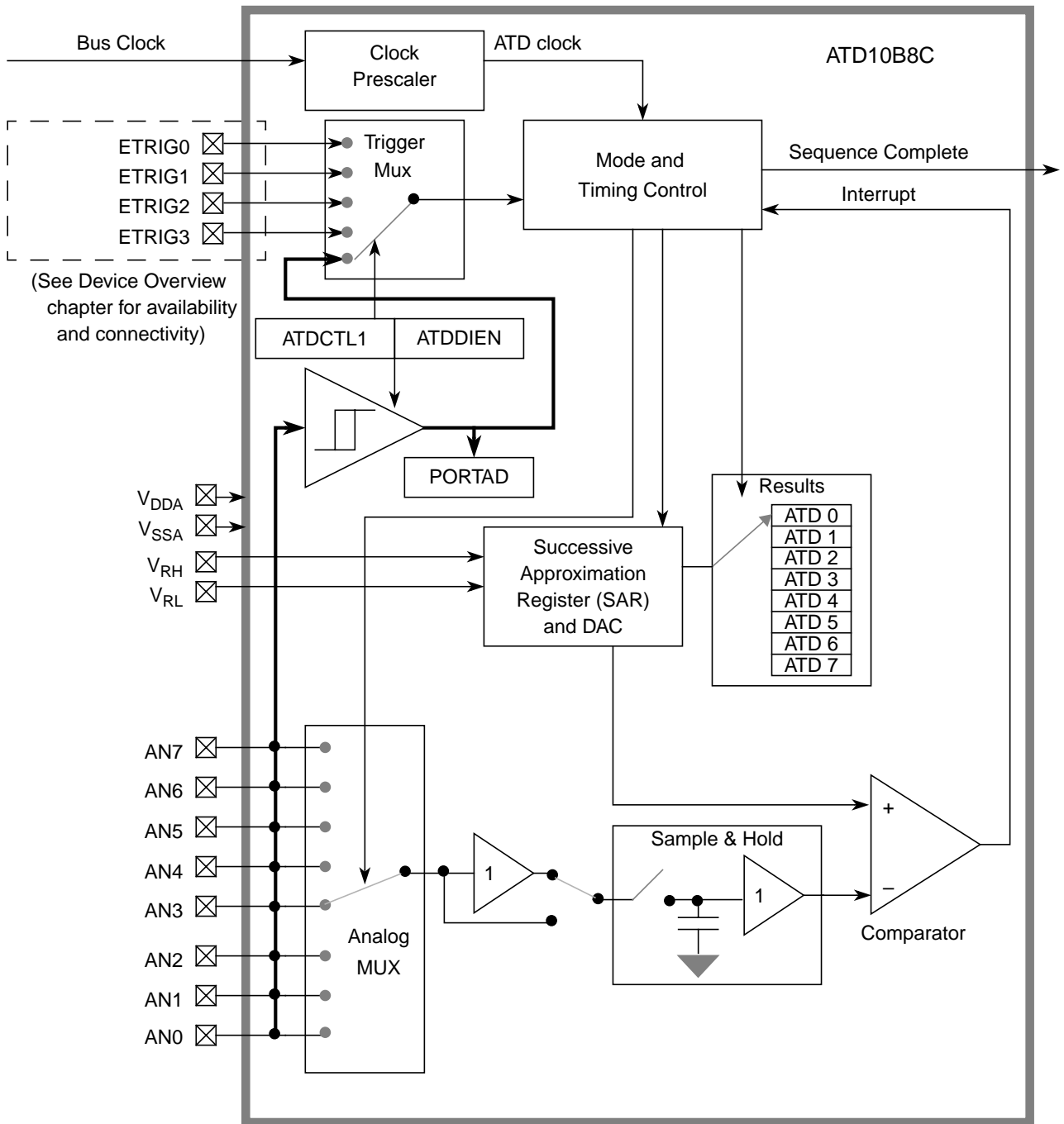
Figure 5-1. ATD Block Diagram
