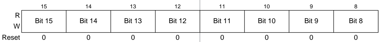
Figure 7-27. Timer Input Capture/Output Compare Register 4 High (TC4)
