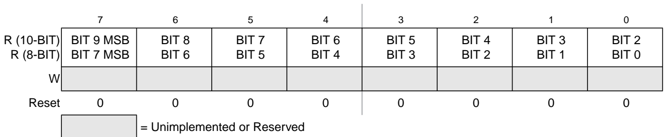
Figure 4-18. Left Justified, ATD Conversion Result Register x, High Byte (ATDDR x H)
