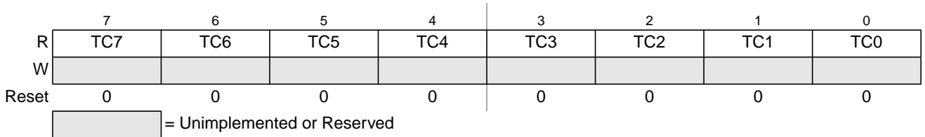
Figure 7-64. Timer Input Capture Holding Register 3 Low (TC3L)
