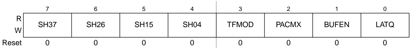
Figure 7-46. Input Control System Register (ICSYS)
