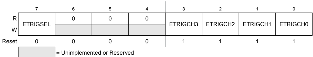
Figure 4-4. ATD Control Register 1 (ATDCTL1)
