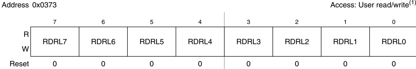
Figure 2-94. Port L Reduced Drive Register (RDRL)
