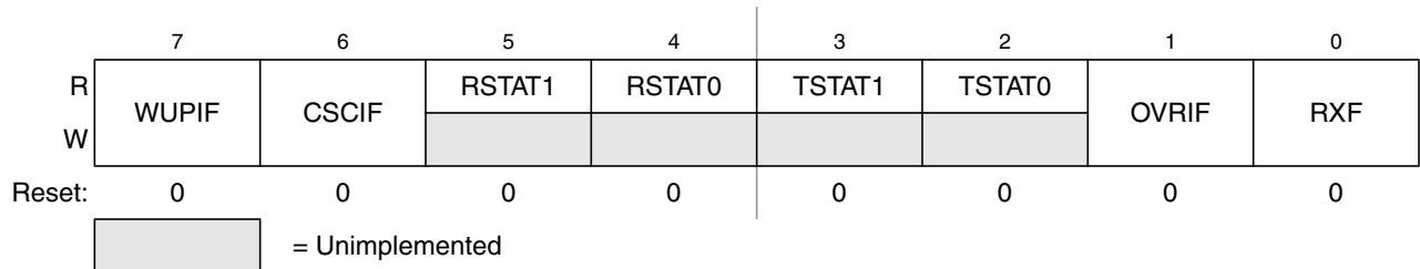
Figure 16-8. MSCAN Receiver Flag Register (CANRFLG)
