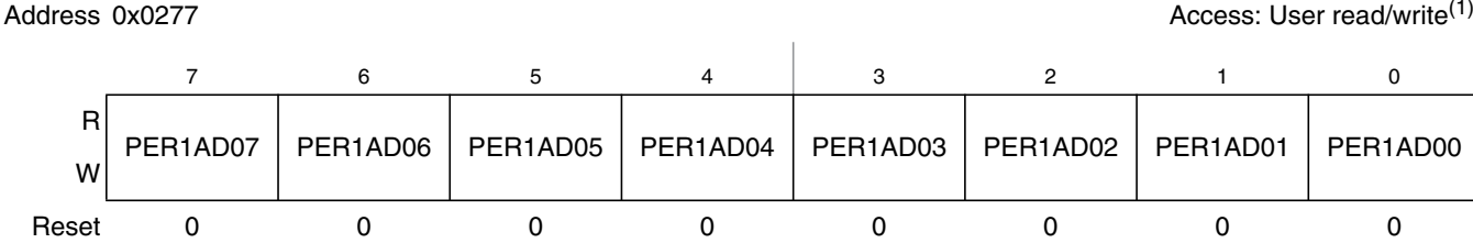
Figure 2-74. Port AD0 Pull Up Enable Register 1 (PER1AD0)
