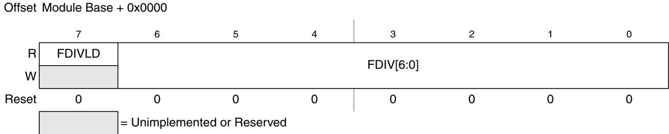
Figure 24-5. Flash Clock Divider Register (FCLKDIV)
