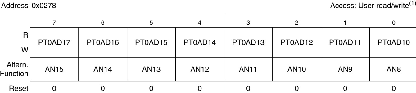
Figure 2-75. Port AD1 Data Register 0 (PT0AD1)
