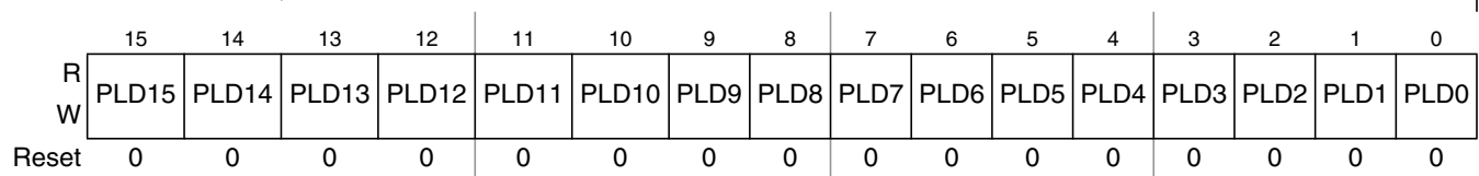
Figure 18-14. PIT Load Register 3 (PITLD3)
