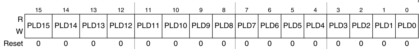
Figure 18-11. PIT Load Register 0 (PITLD0)
