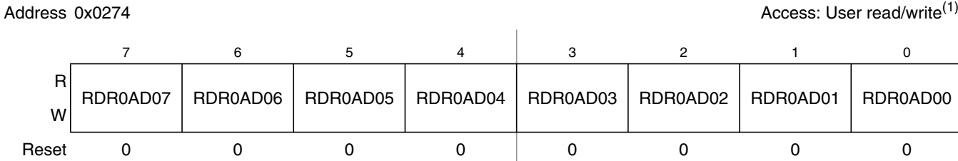
Figure 2-71. Port AD0 Reduced Drive Register 0 (RDR0AD0)
