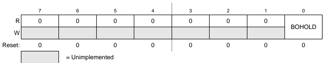
Figure 12-17. MSCAN Miscellaneous Register (CANMISC)
