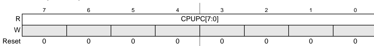
Figure 3-7. Captured S12ZCPU Program Counter (MMCPCH, MMPCPM, MMCPCL)
