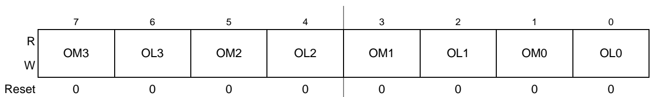
Figure 11-11. Timer Control Register 2 (TCTL2)
