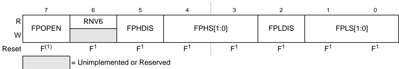
Figure 19-14. Flash Protection Register (FPROT)
