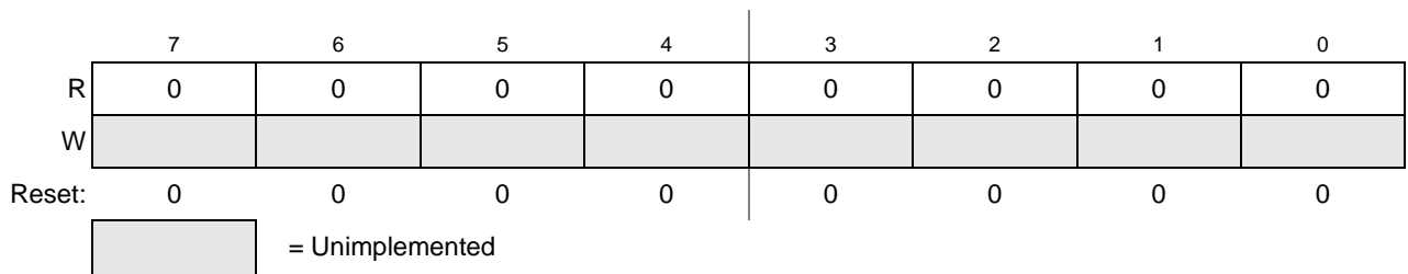
Figure 12-16. MSCAN Reserved Register
