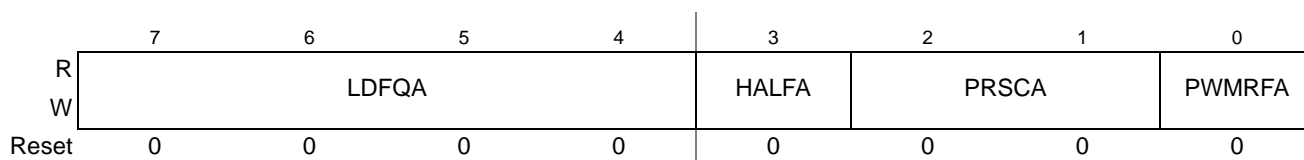
Figure 14-25. PMF Frequency Control A Register (PMFFQCA)
