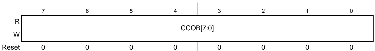
Figure 19-28. Flash Common Command Object 4 Low Register (FCCOB4LO)
