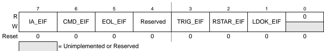
Figure 9-12. ADC Error Interrupt Flag Register (ADCEIF)
