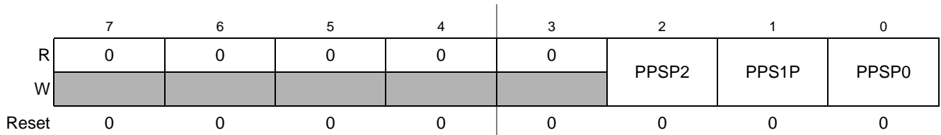
Figure 2-22. Port P Polarity Select Register
