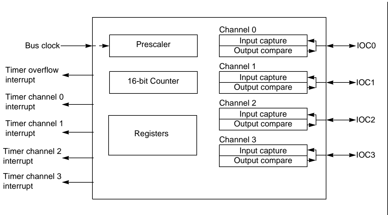
Figure 11-1. TIM16B4CV3 Block Diagram
