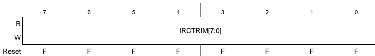
Figure 8-28. S12CPMU_UHV_V6 IRC1M Trim Low Register (CPMUIRTRIML)
