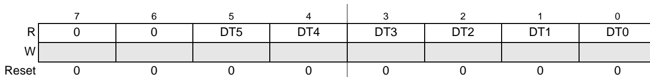
Figure 14-15. PMF Deadtime Sample Register (PMFDTMS)
