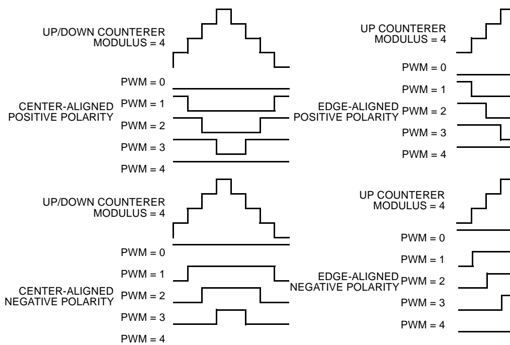
Figure 14-67. PWM Polarity
