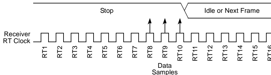
Figure 15-29. Fast Data
