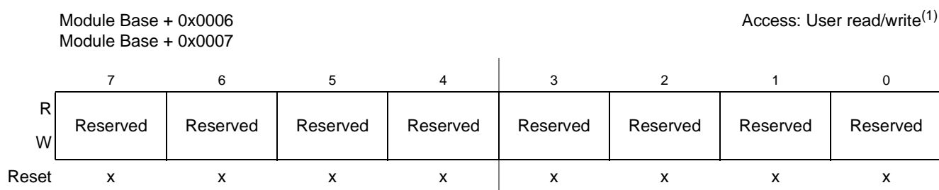
Figure 10-8. Reserved Register
