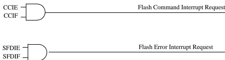
Figure 19-32. Flash Module Interrupts Implementation
