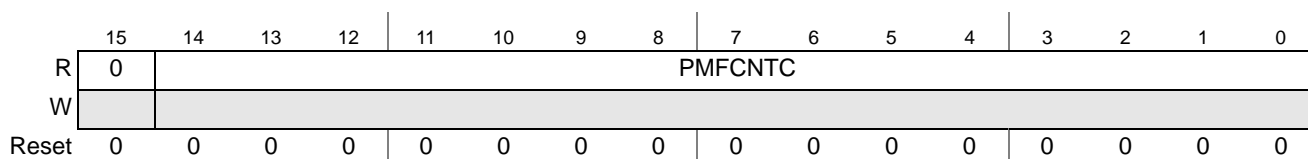
Figure 14-36. PMF Counter C Register (PMFCNTC)
