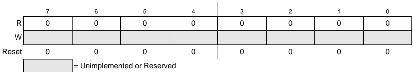
Figure 19-18. Flash Reserved1 Register (FRSV1)
