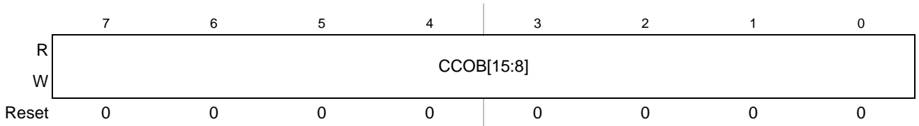
Figure 19-25. Flash Common Command Object 3 High Register (FCCOB3HI)
