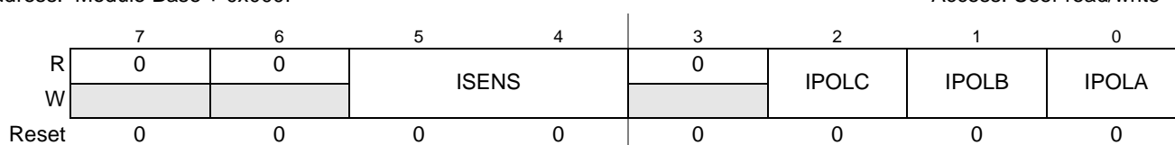
Figure 14-16. PMF Correction Control Register (PMFCCTL)
