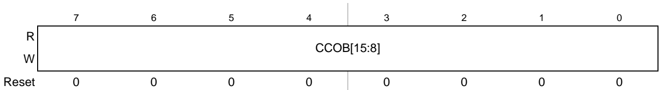
Figure 19-27. Flash Common Command Object 4 High Register (FCCOB4HI)
