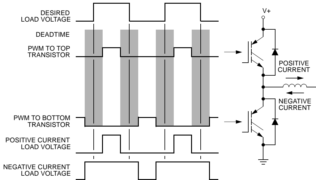
Figure 14-54. Deadtime Distortion
