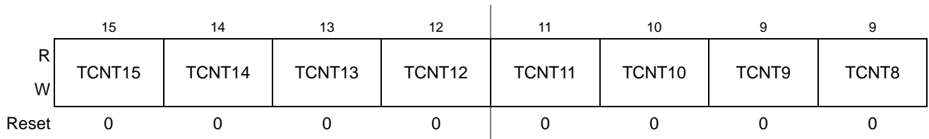
Figure 11-6. Timer Count Register High (TCNTH)
