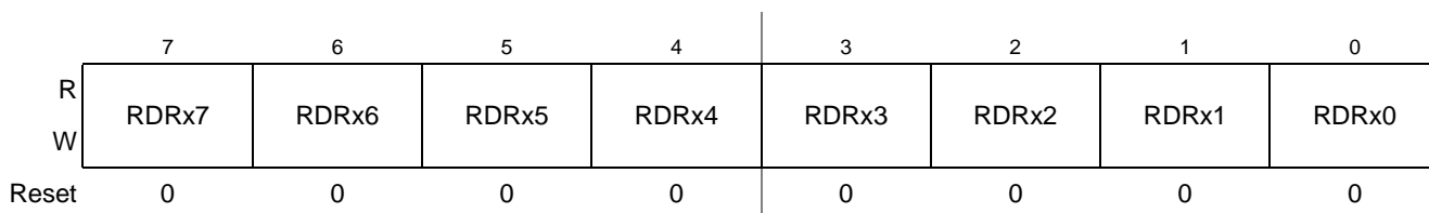
Figure 2-19. Reduced Drive Register
