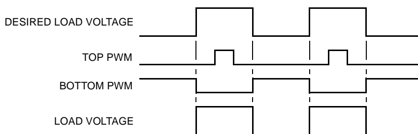
Figure 14-61. Correction with Negative Current
