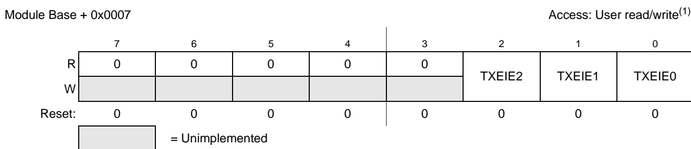
Figure 12-11. MSCAN Transmitter Interrupt Enable Register (CANTIER)
