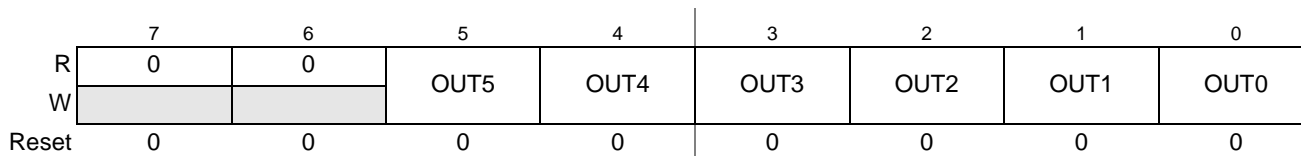
Figure 14-14. PMF Output Control Bit Register (PMFOUTB)
