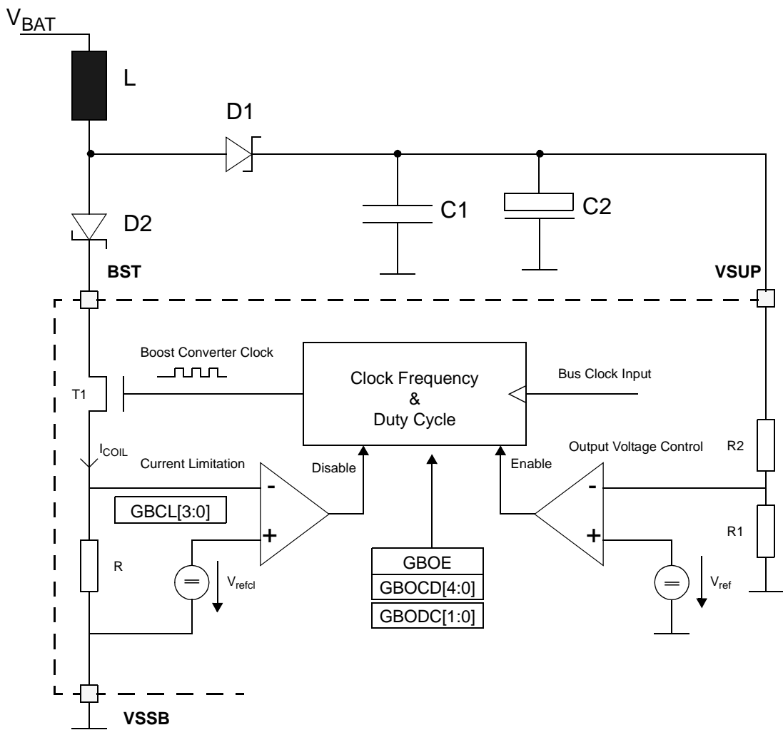
Figure 17-25. Boost Converter Option with external Components 1
