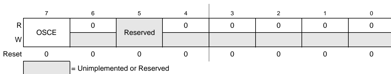
Figure 8-31. S12CPMU_UHV_V6 Oscillator Register (CPMUOSC)
