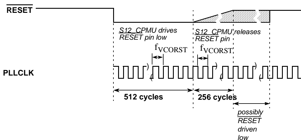
Figure 8-40. RESET Timing
