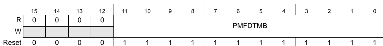
Figure 14-33. PMF Deadtime B Register (PMFDTMB)
