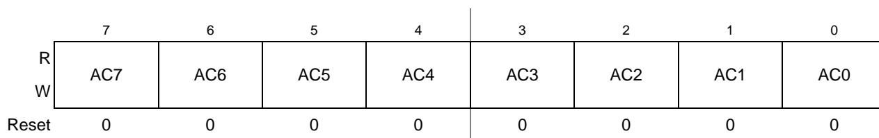
Figure 12-21. MSCAN Identifier Acceptance Registers (Second Bank) — CANIDAR4–CANIDAR7
