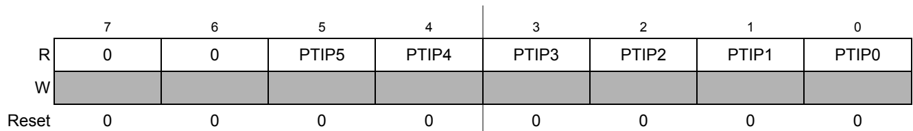
Figure 2-36. Port P Input Register (PTIP)
