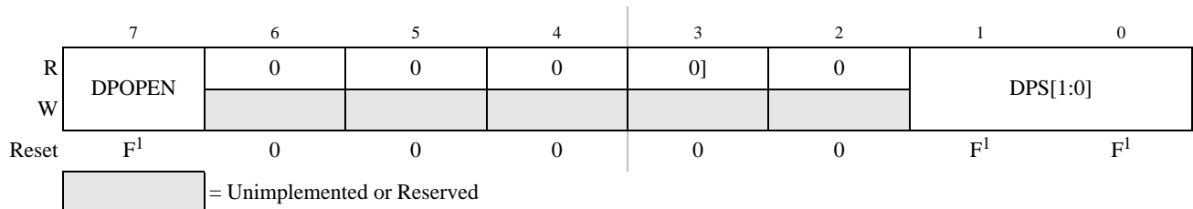
Figure 18-15. EEPROM Protection Register (DFPROT)
