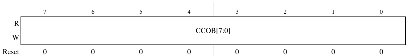
Figure 20-28. Flash Common Command Object 5 Low Register (FCCOB5LO)
