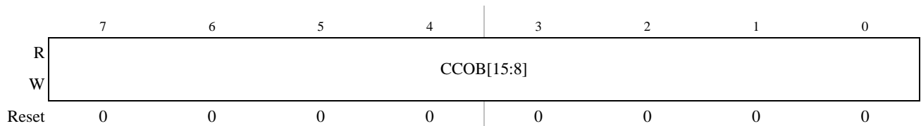
Figure 18-24. Flash Common Command Object 3 High Register (FCCOB3HI)
