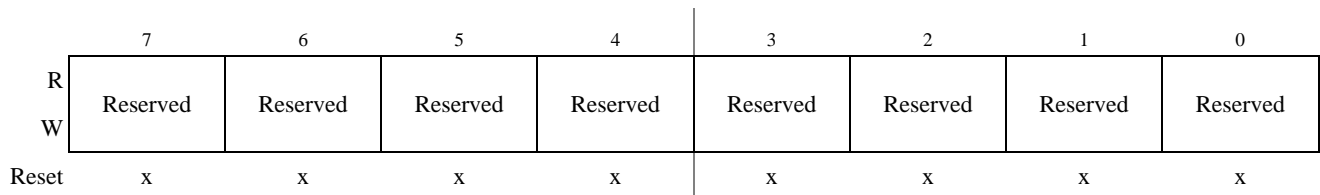
Figure 2-9. Reserved Register
