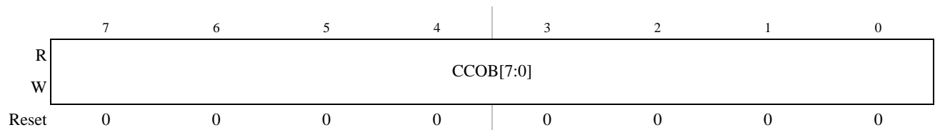
Figure 19-18. Flash Common Command Object 0 Low Register (FCCOB0LO)
