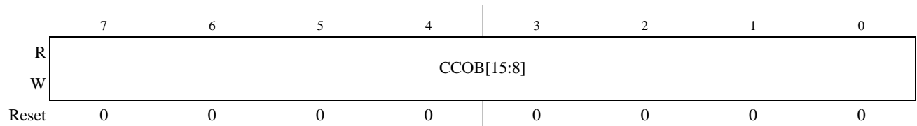
Figure 19-17. Flash Common Command Object 0 High Register (FCCOB0HI)
