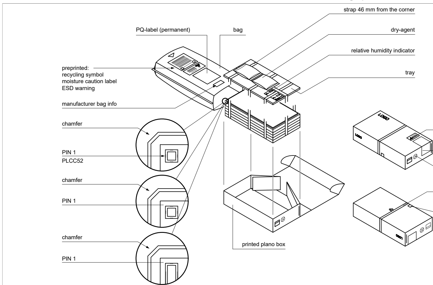
Figure 32. Packing information 5 tray
