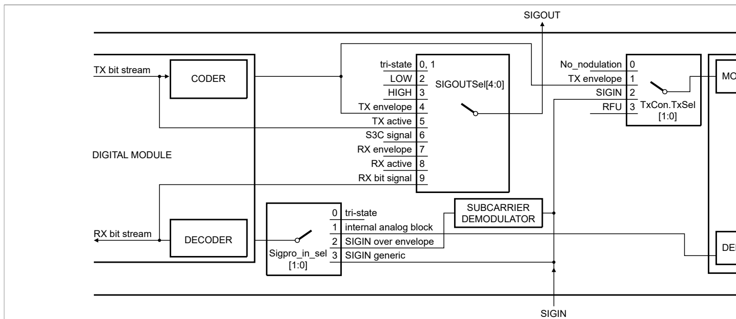
Figure 23. Overview SIGIN/SIGOUT Signal Routing
