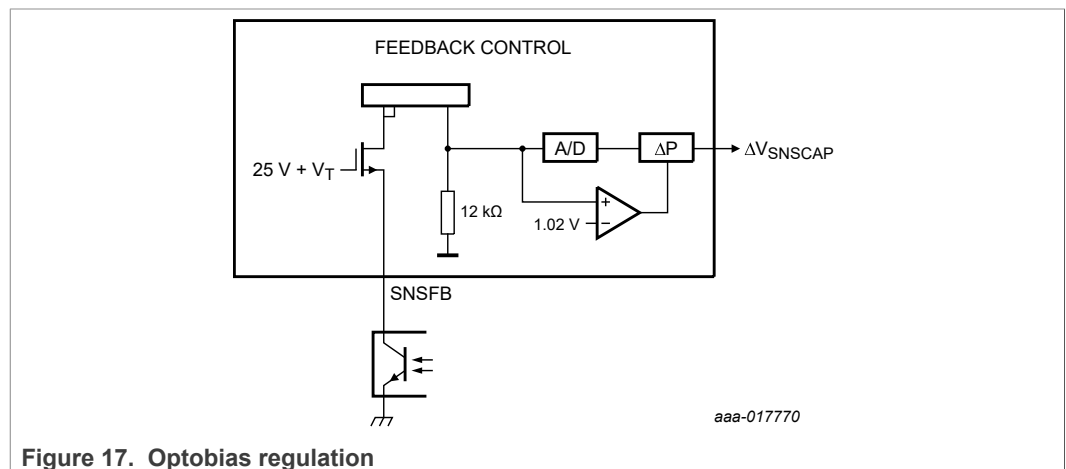
Figure 17. Optobias regulation
