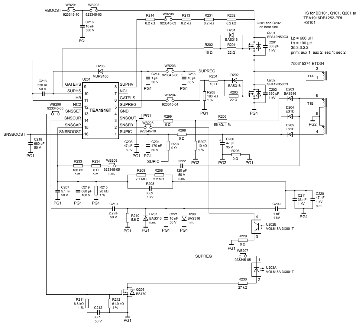
Figure 23. Schematic TEA1916DB1262 240 W prototype demo board (LLC)
