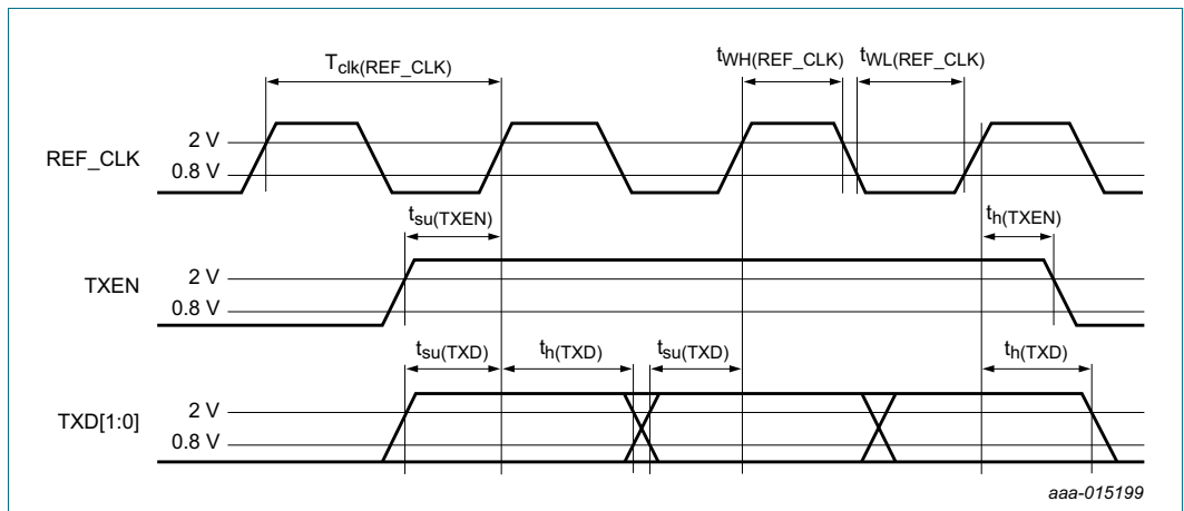
Fig 14. RMII transmit timing diagram
