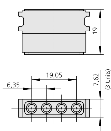
Module, 4 Positions
