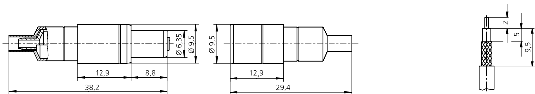
Strip off length
