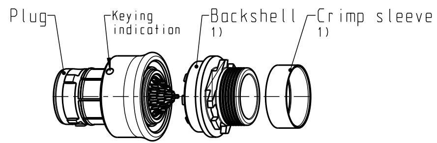
Delivery condition 1:1
