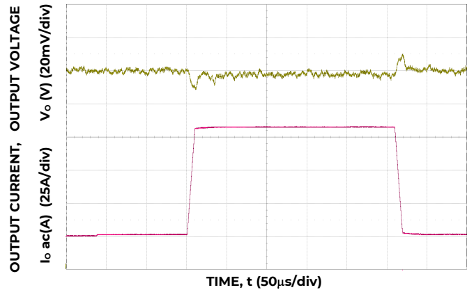
Figure 16. Trans. Resp. to 100A/µs Load Change from 25% to 75% at 12VIN, C_o=4 \times 0.047 \mu\text{F} + 4 \times 0.1 \mu\text{F} + 15 \times 22 \mu\text{F} + 73 \times 47 \mu\text{F} + 6 \times 470 \mu\text{F} polymer.
