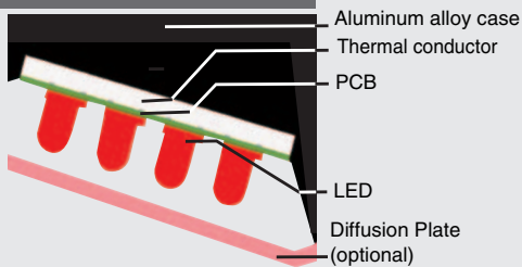
Cross-sectional Diagram
