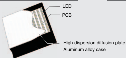
Cross-sectional Diagram
