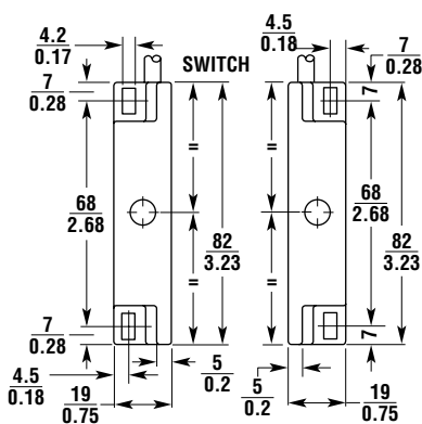
Switch - Type 2
