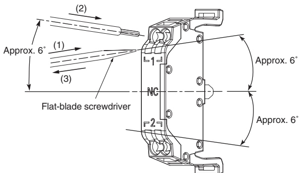
The wiring and screwdriver angles for the Lighting Unit and Switch Block (2 contacts) are the same as for the Switch Block (1 contact) shown in the above illustration.
