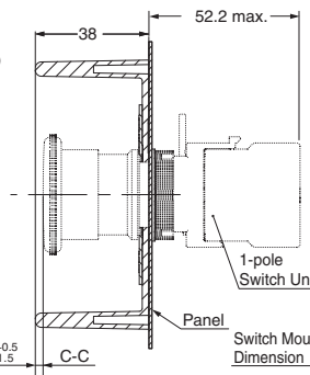
Screw Terminal Block Type Mounting a 1-pole Switch Unit
