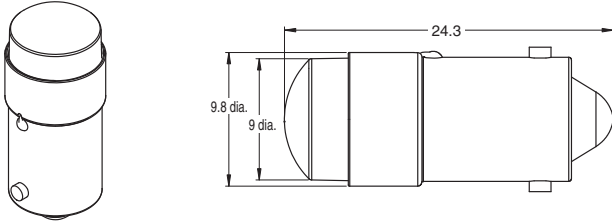
LED Lamps A22NZ-L-□□
