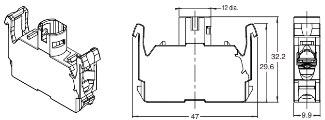
Lighting Units A22NZ-T-□
