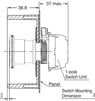
Push-in Plus Terminal Block Type Mounting a 1-pole Switch Unit
