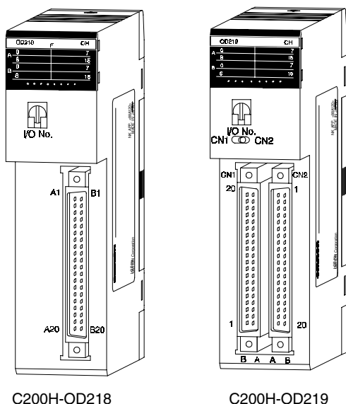
C200H-OD218
