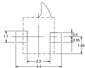
PCB land dimensions (reference) (TOP VIEW)
