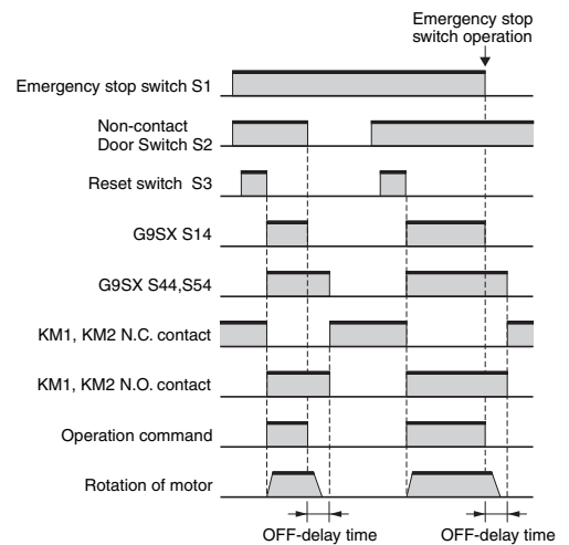
Timing chart
