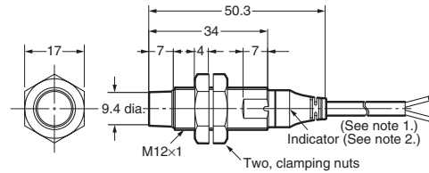
E2A-M12KN08-WP-□□
