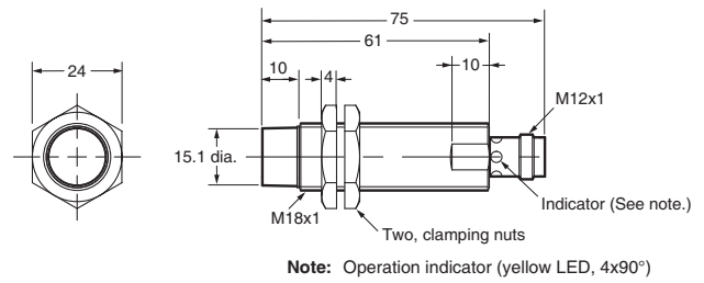
E2A-S18LN16-M1-□
