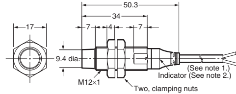
E2A-M12KN08-WP-□□
