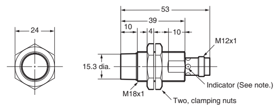
E2A-S18KN16-M1-□
