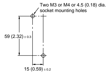
Mounting holes
