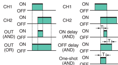
2. Control Output (AND, OR, Sync) and Timing Chart for Timer Settings (T: Set Time)
